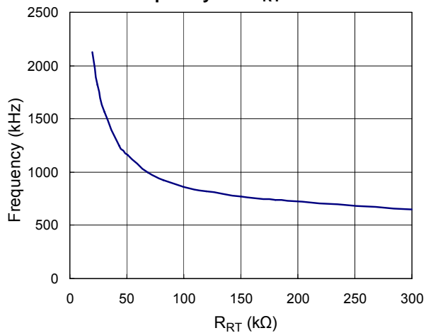
Frequency vs. R RT Resistor
