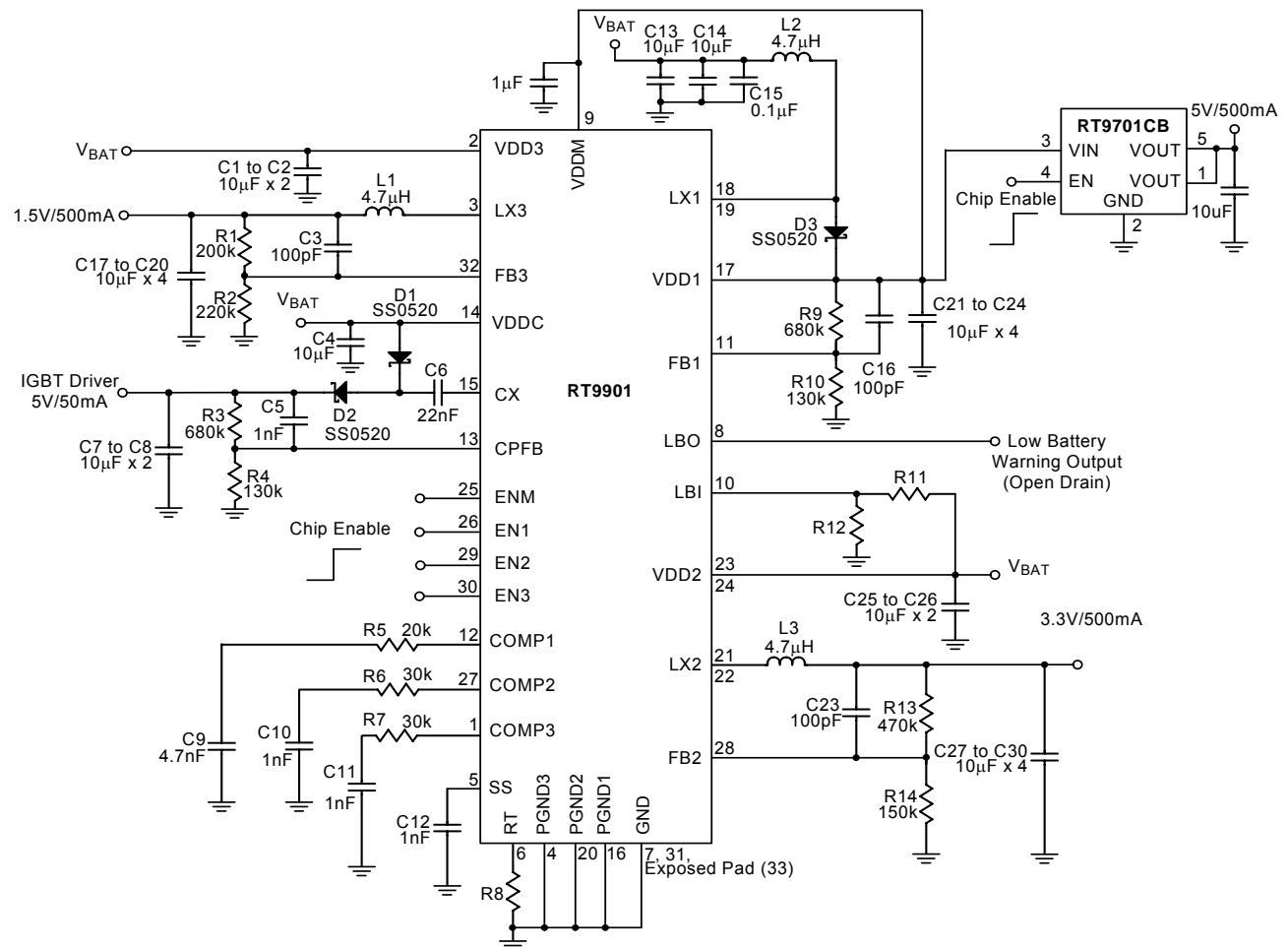
Figure 1. Typical Application Circuit from 1-cell Li+ Battery
