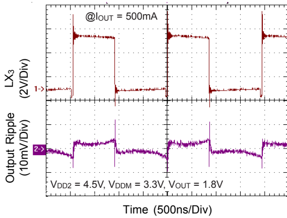
Buck3 LX & Output Ripple
