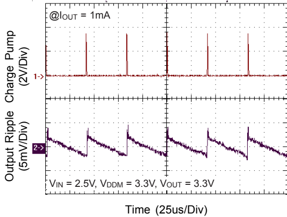
Charge Pump CX & Output Ripple
