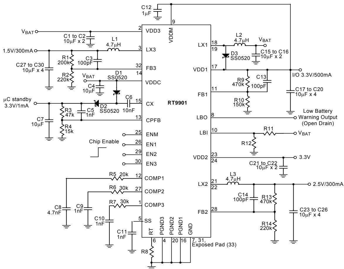
Figure 2. Typical Application Circuit from 2-AA Battery Supply
