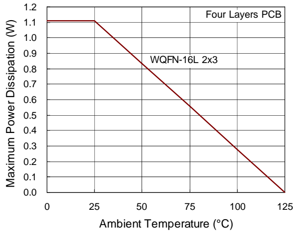
Figure 1. Derating Curve for RT9379 Package
