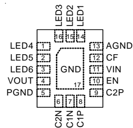
WQFN-16L 2x3
