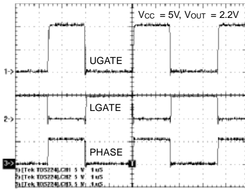
Time (1us/Div)
