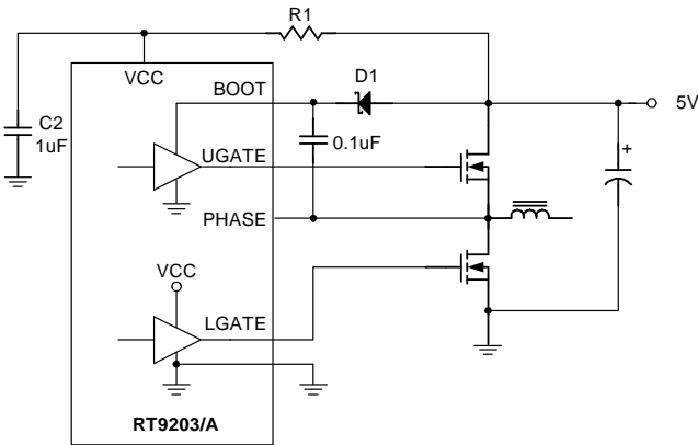
Figure 3. Single 5V power Supply Operation
