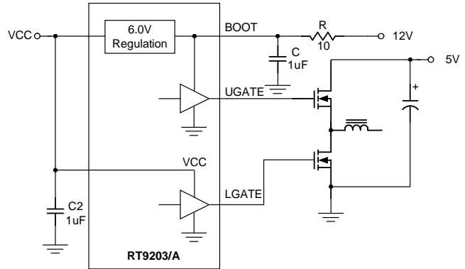
Figure 4. Dual Power Supply Operation
