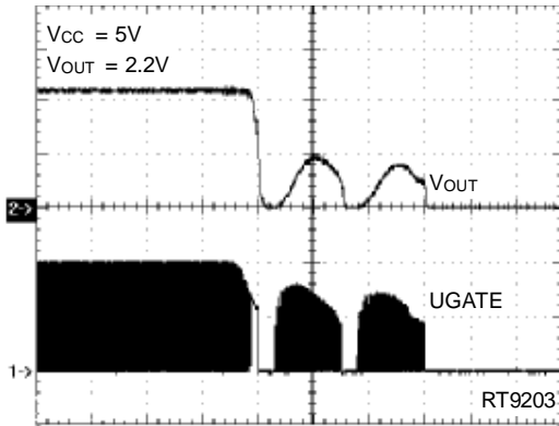
Time (2ms/Div)
