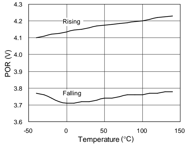
POR (Rising/Falling) vs. Temperature
