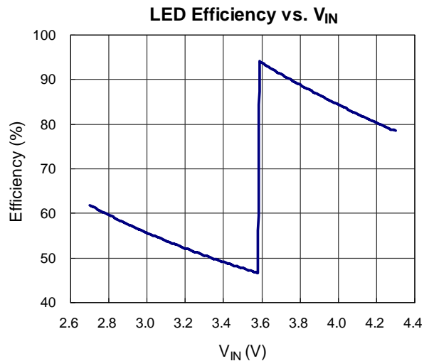
Figure 7. Efficiency of RT9363A. ( I_{LED} = 60mA , V_F = 3.5V )
