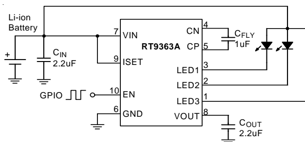
Figure 2. Internal R_{SET(MAX)} = 20mA , for 2-WLEDs Application Circuit
