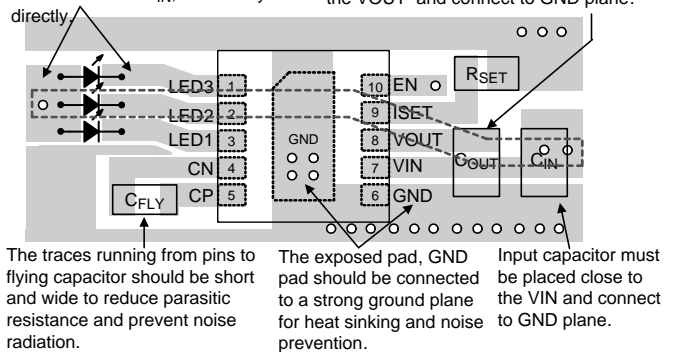
Figure 8. PCB Layout Guide
