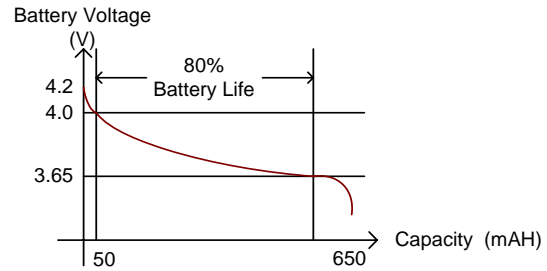
Figure 6. Li-ion Battery Energy Capacity Versus Battery Voltage.
