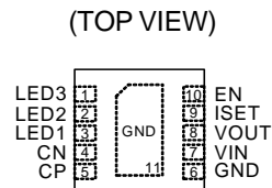
WDFN-10L 3x3
