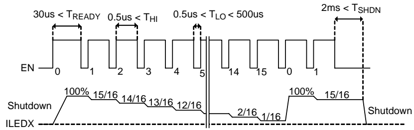
Figure 5. Pulse Dimming Waveform
