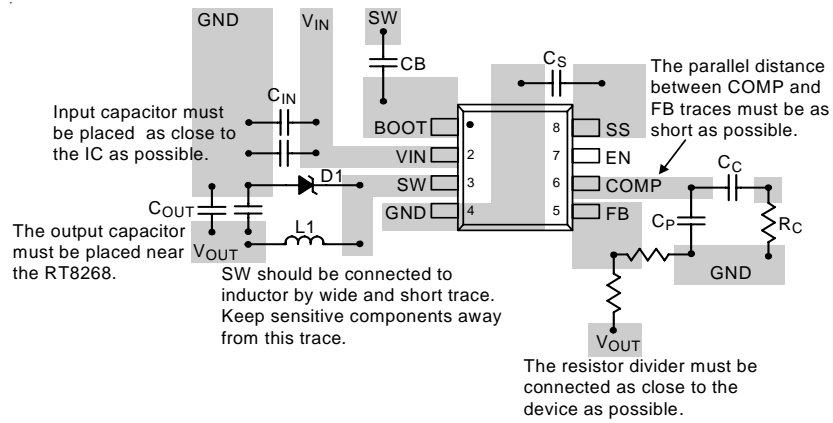
Figure 5. PCB Layout Guide for SOP-8
