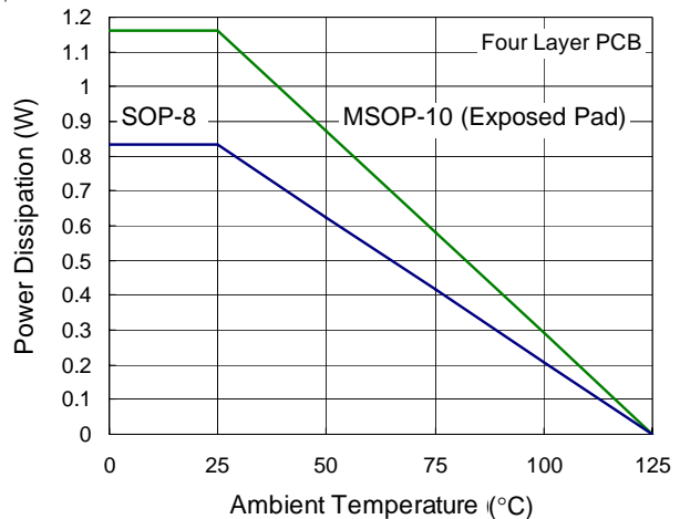
Figure 3. Derating Curves for RT8268 Packages
