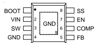
SOP-8 (Expoaed Pad)
