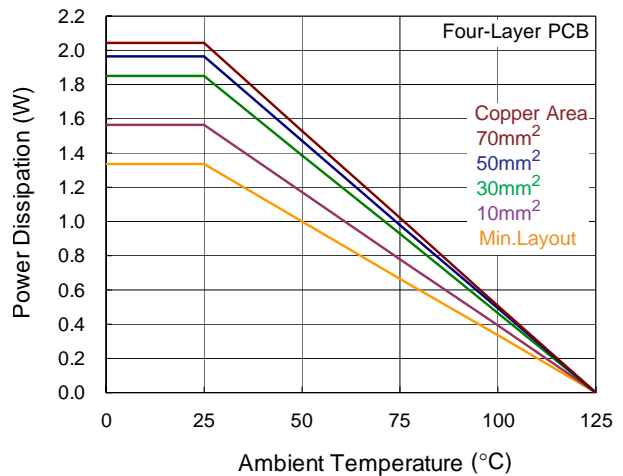
Figure 7. Derating Curves for RT8253B Package
