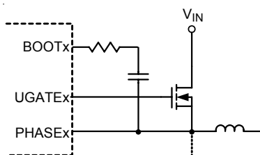
Figure 5. Reducing the UGATEx Rise Time
