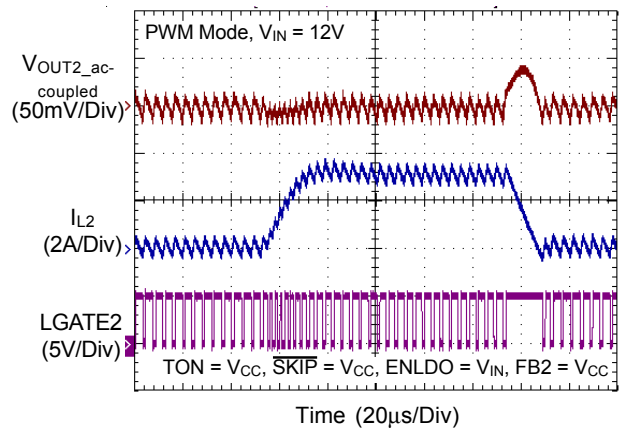
VOUT2 Load Transient Response
