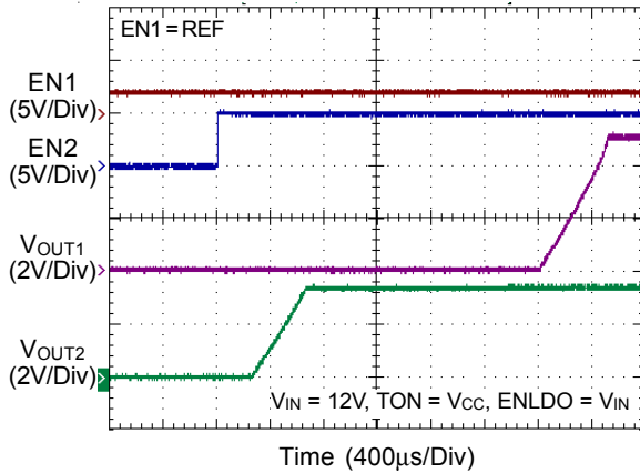
Power On from EN2 (Delay Start)
