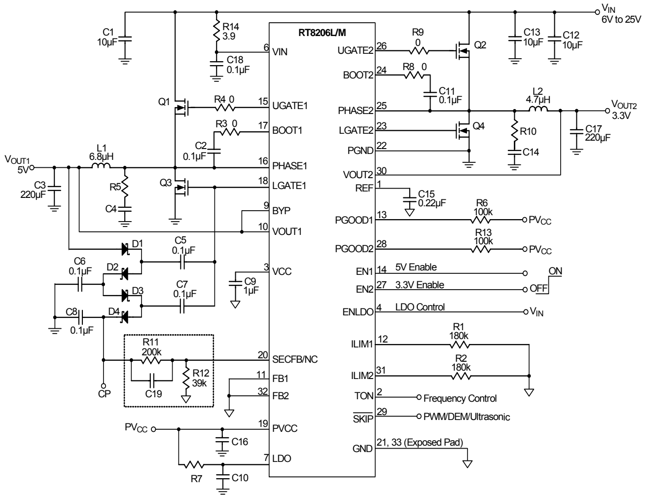
Figure 1. Fixed Voltage Regulator
