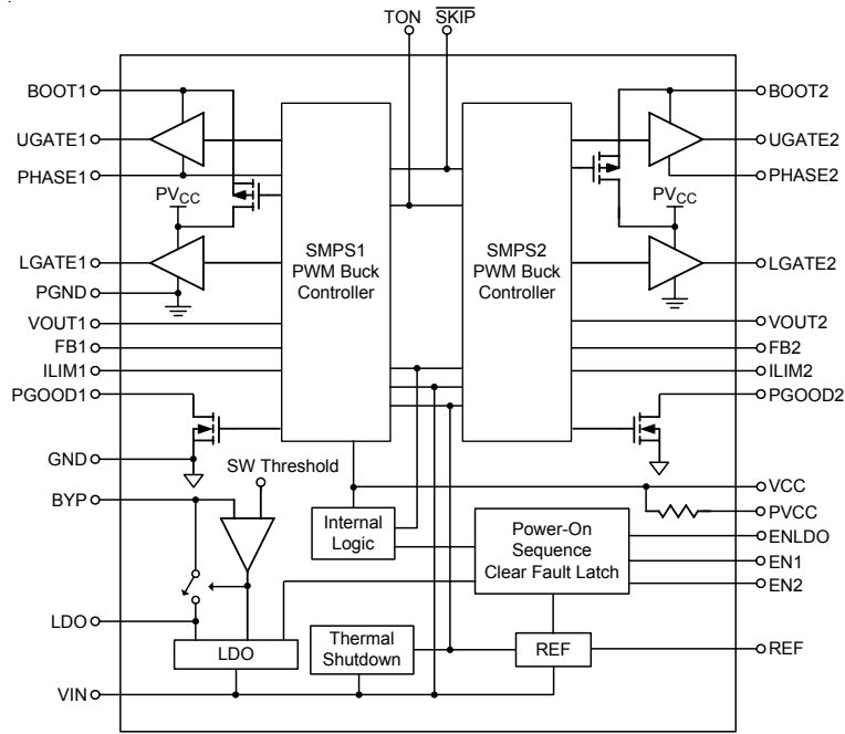
Function Block Diagram
