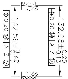
SECTION J-J
