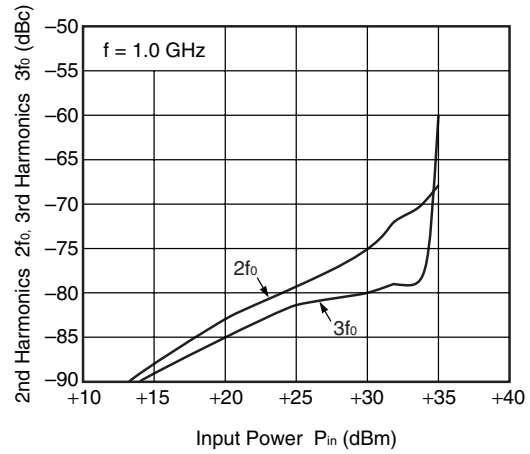
2ND HARMONICS, 3RD HARMONICS vs. INPUT POWER
