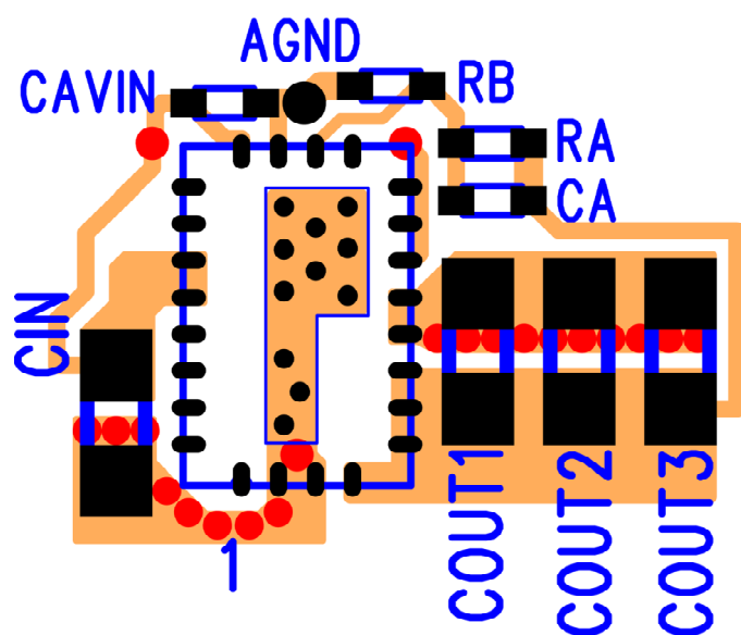
Figure 8. Optimized Layout Recommendations
