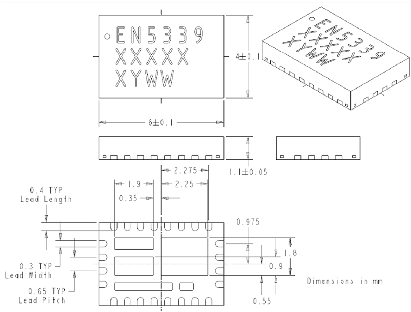
Figure 11. EN5339QI Package Dimensions (Bottom View)
