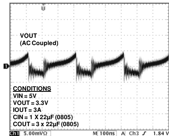
Output Ripple at 500MHz
