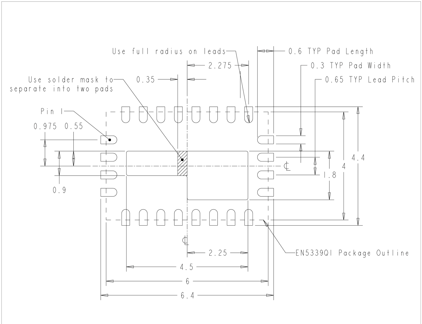
Figure 10. Recommended PCB Footprint (Top View)
