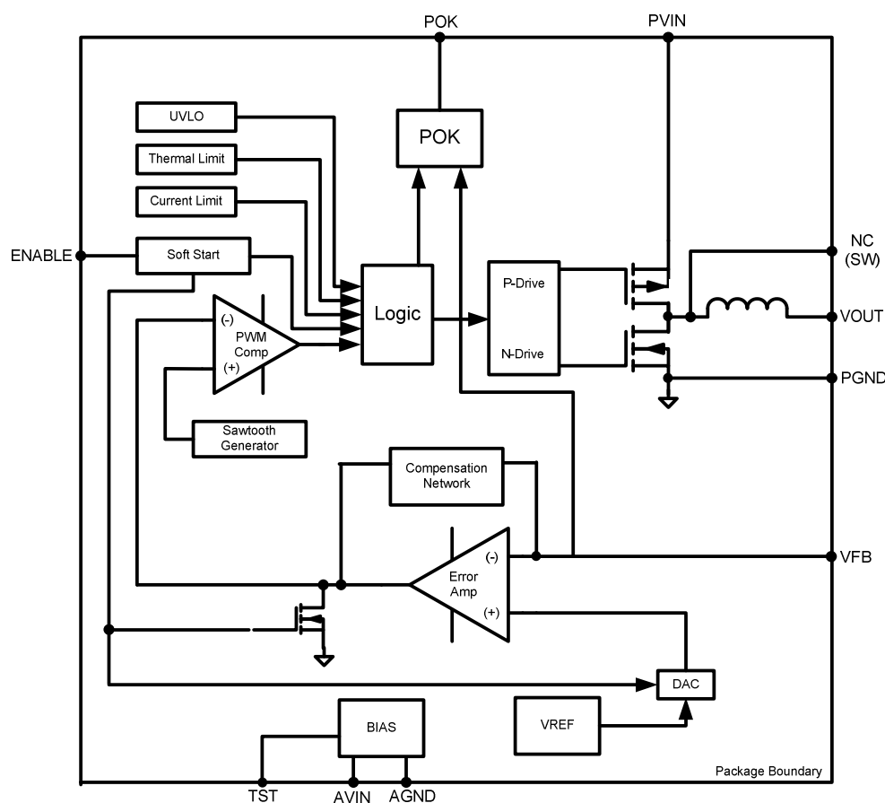
Figure 4: Functional Block Diagram
