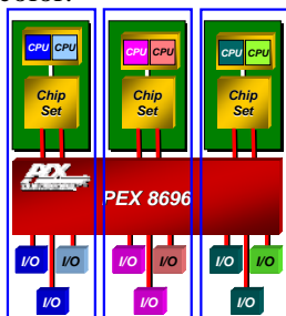
Figure 7. Multi-Host System
