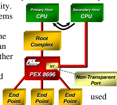
Figure 3. Non-Transparent Port
