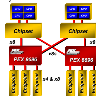
Figure 9. Host Fail-Over
