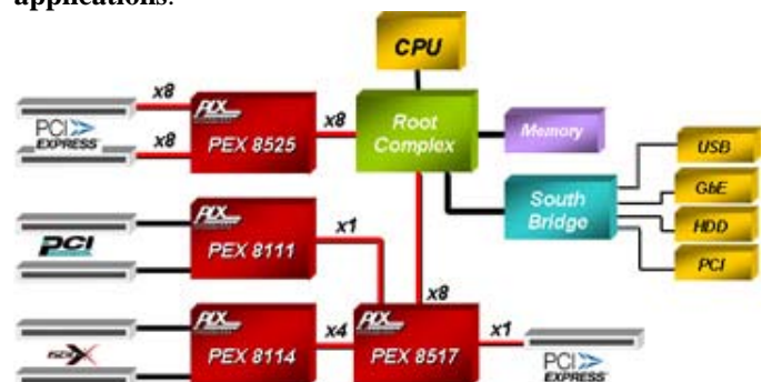
Figure 2. Fan-in/out Usage
