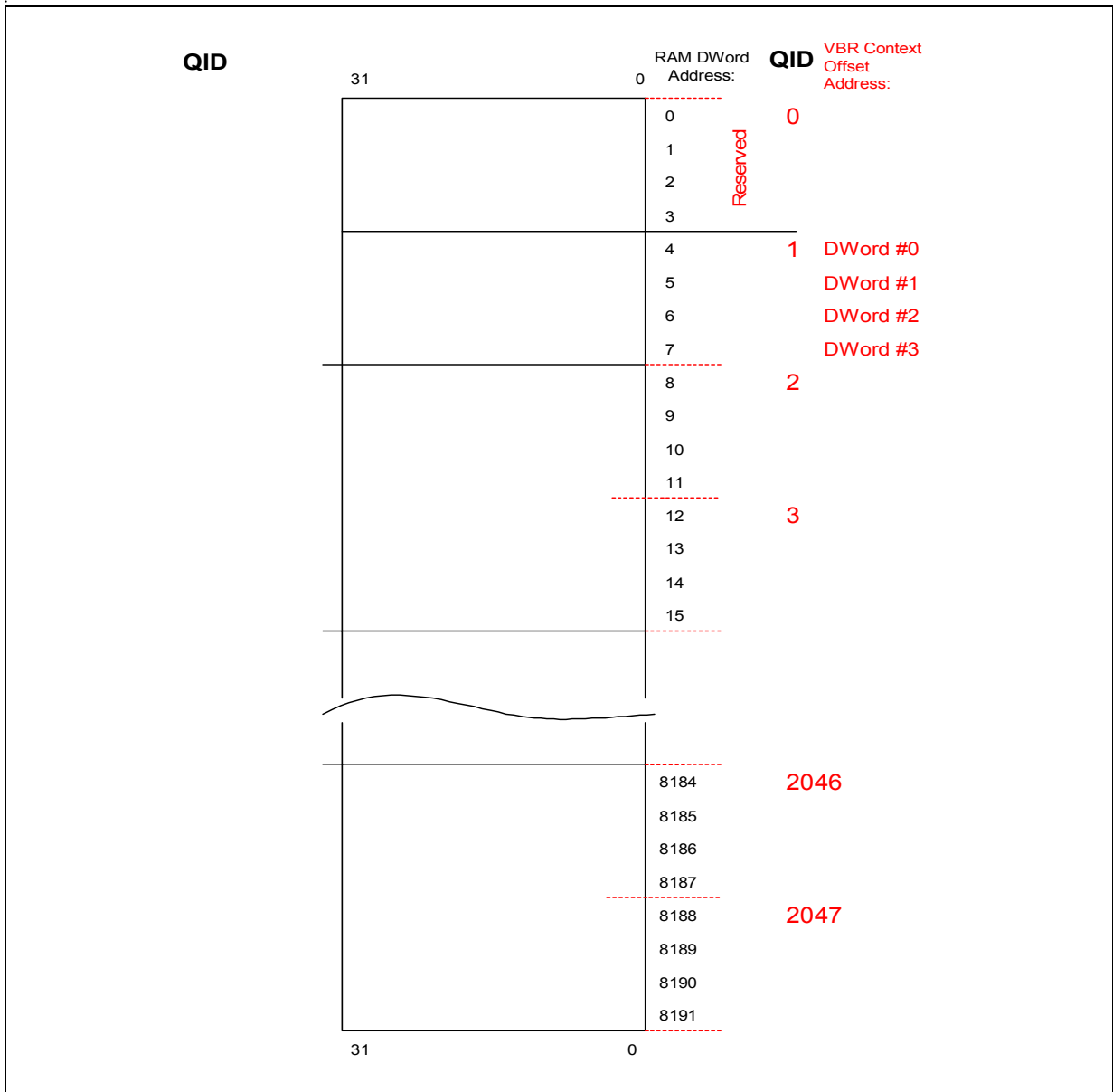
Figure 3-37 AVT Context RAM Addressing Scheme
