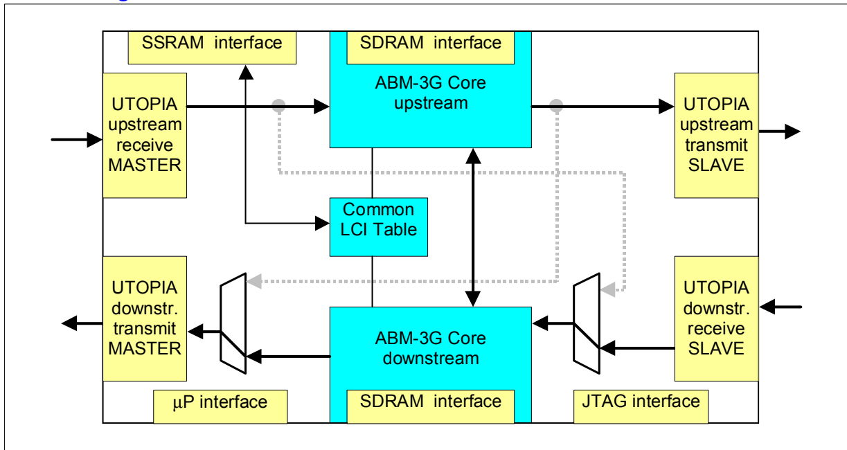
Figure 3-10 ABM-3G in Bi-directional Mode
