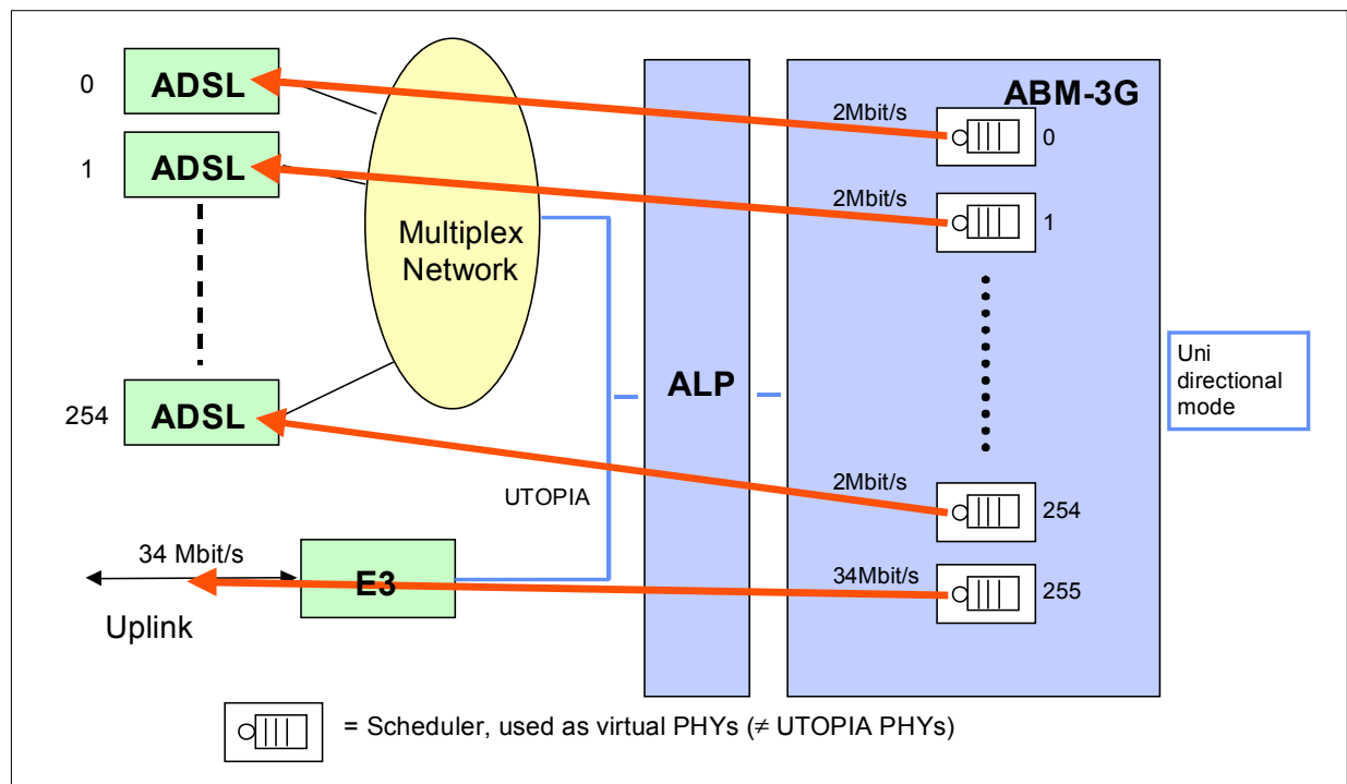
Figure 4-7 ABM-3G Application Example: DSLAM
