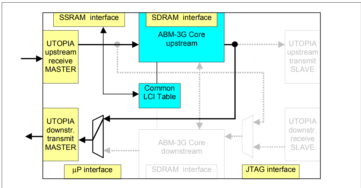
Figure 3-12 ABM-3G in Uni-directional Mode Using one Core
