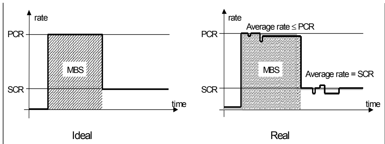
Figure 3-28 Ideal and Real ABM-3G Shaper Output
