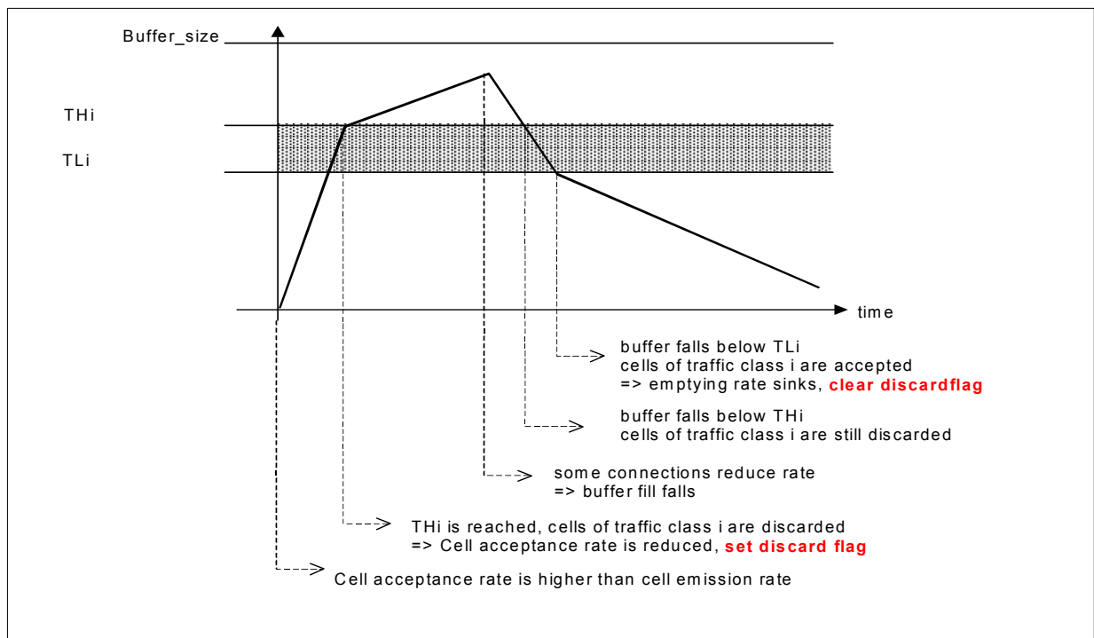
Figure 3-19 Buffer Threshold with Hysteresis
