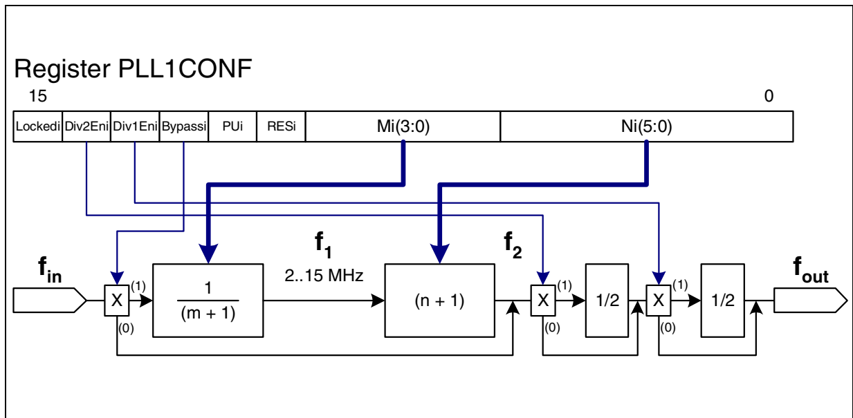
Figure 3-8 DPLL Structure
