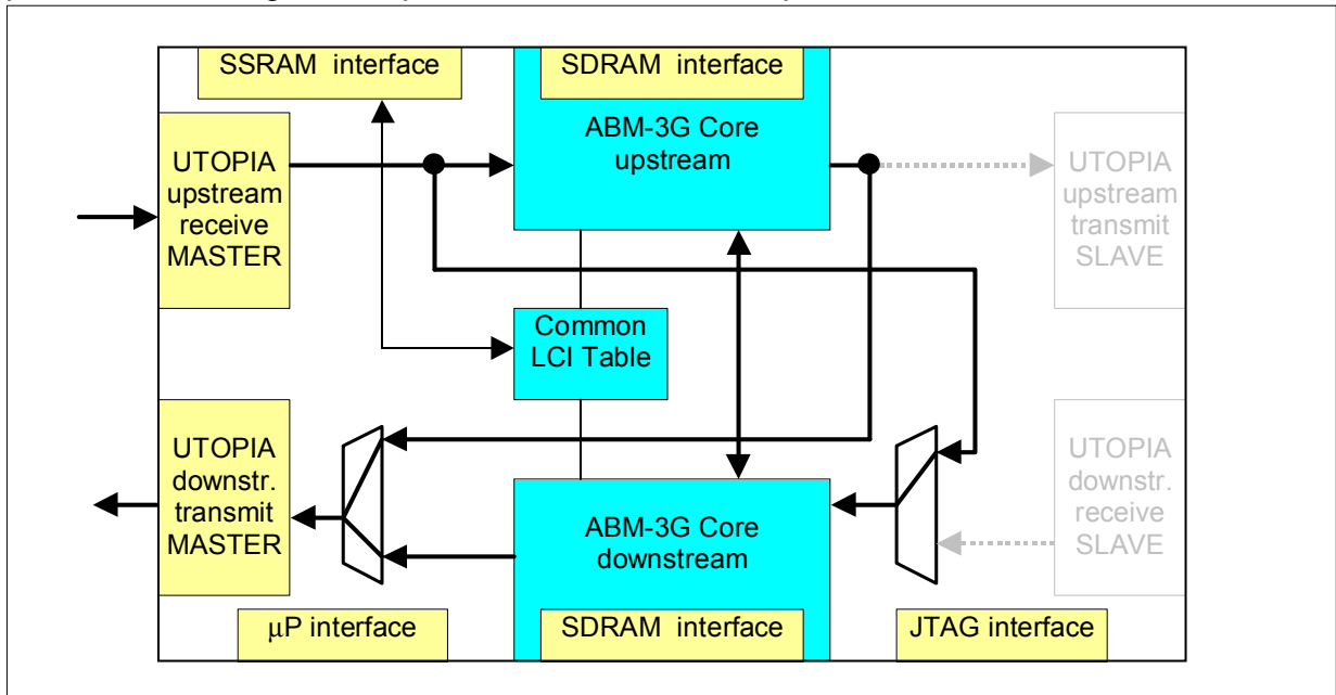
Figure 3-11 ABM-3G in Uni-directional Mode Using both Cores
