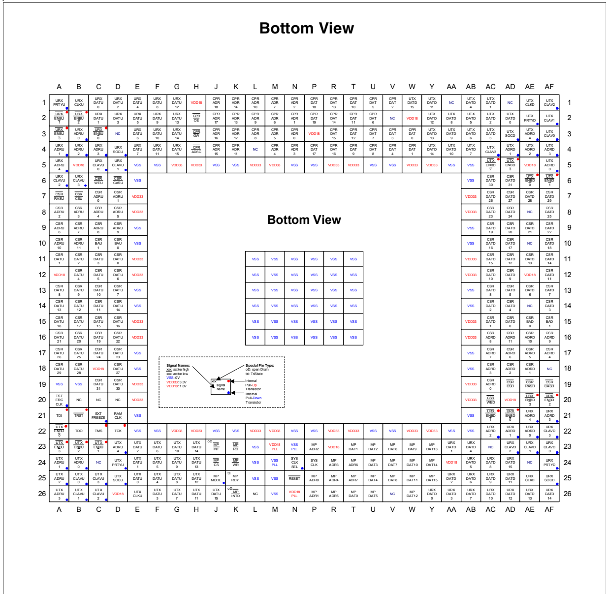
Figure 2-1 Pin Configuration (Bottom View)
