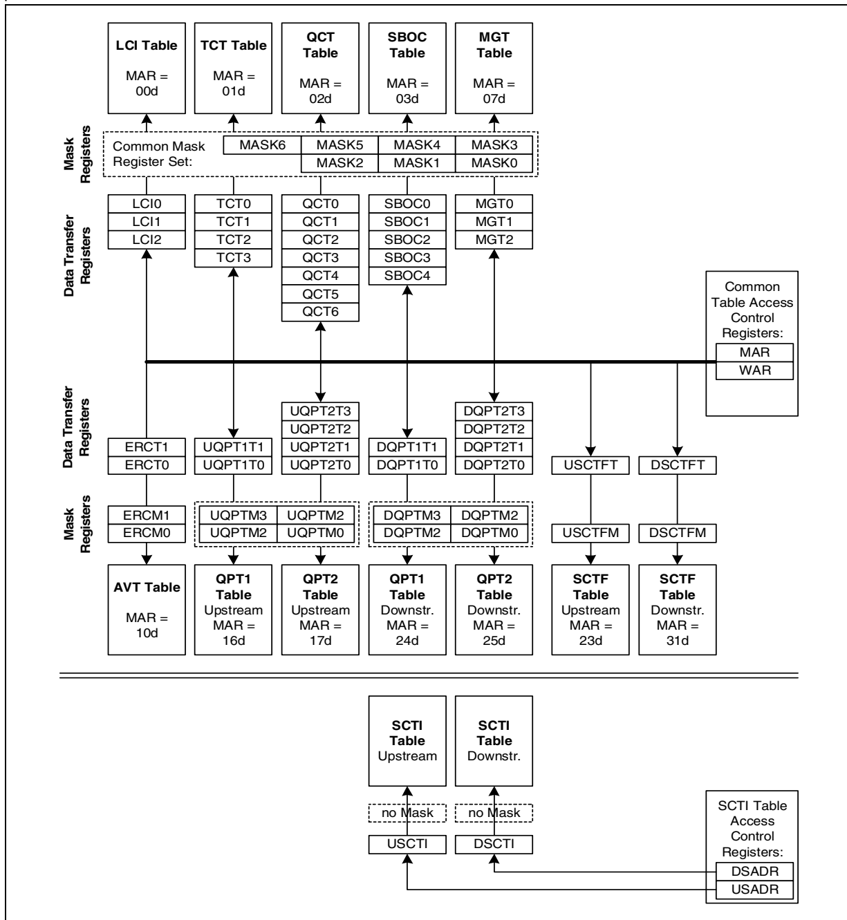
Figure 3-36 Table Access Overview
