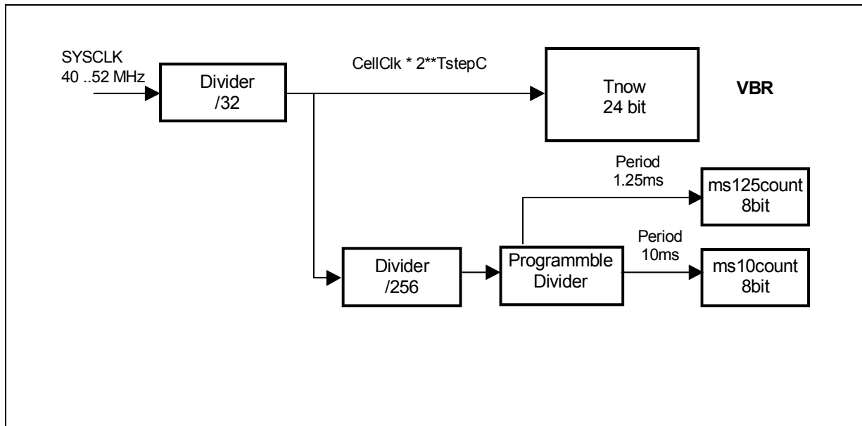
Figure 3-34 SCAN Timer Generation
