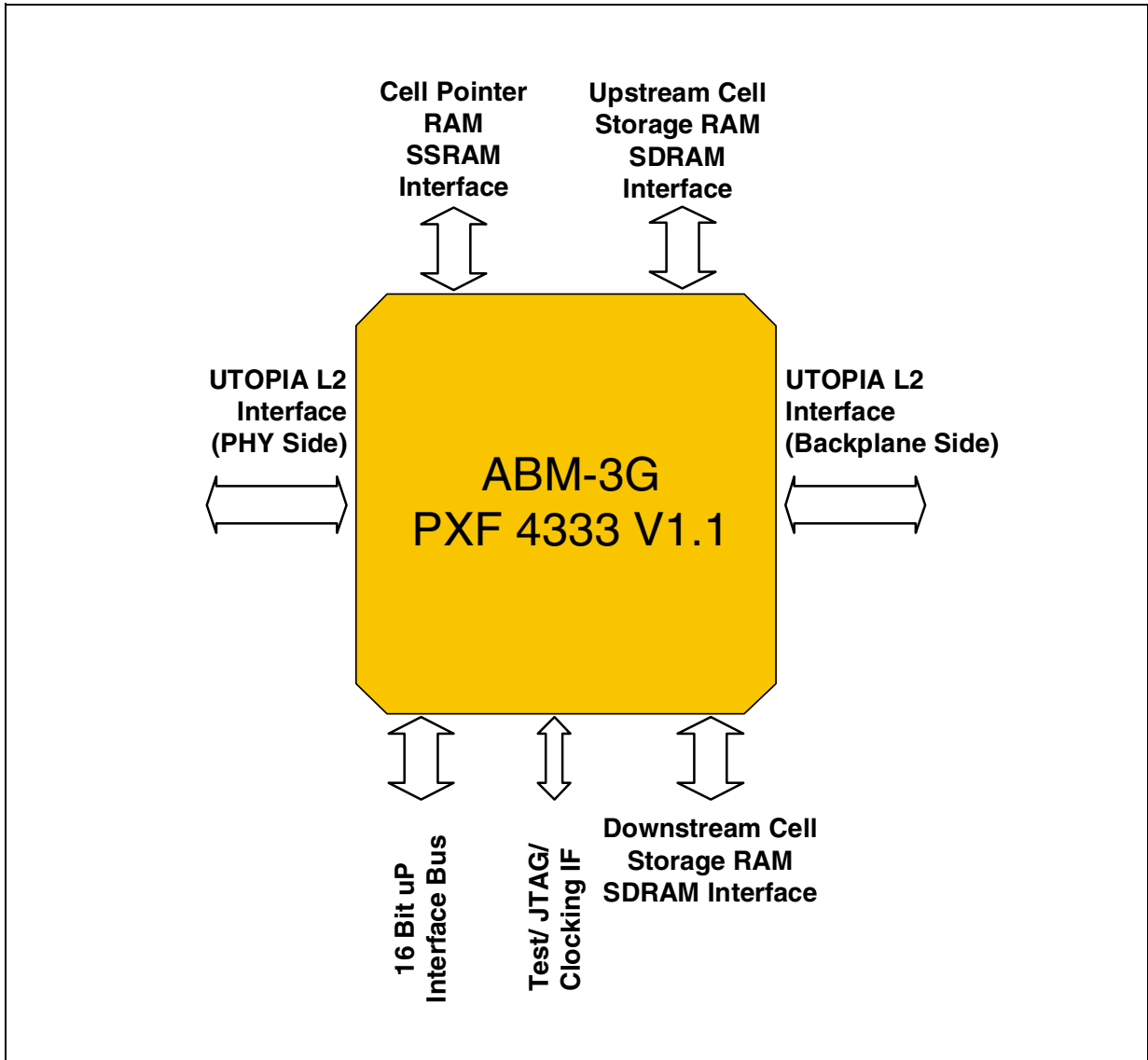
Figure 1-1 Logic Symbol
