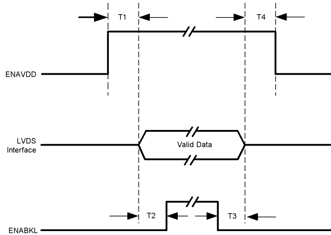
FIGURE 23. Sample LCD Power Up Sequence
