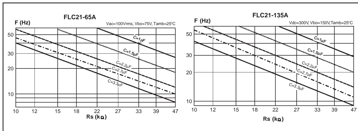
Fig. 4: Spark frequency versus Rs and C
