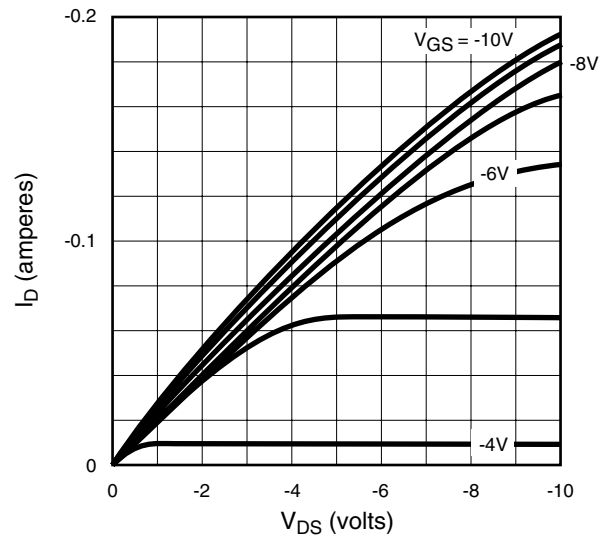
Saturation Characteristics
