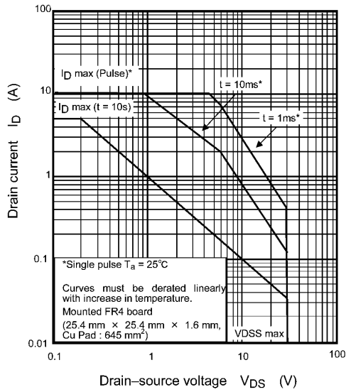
Fig. 7.15 Safe Operating Area
