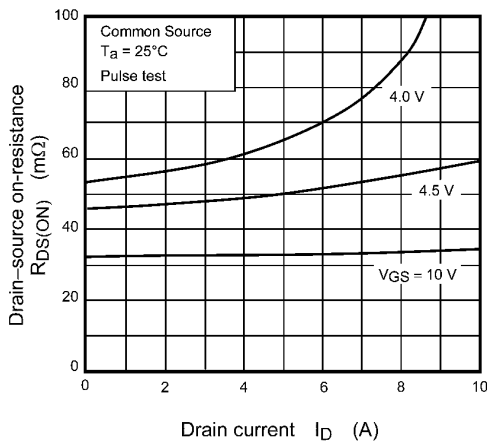
Fig. 7.5 R_{DS(ON)} - I_D
