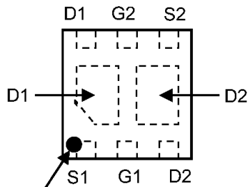
Fig. 6.1 Marking
