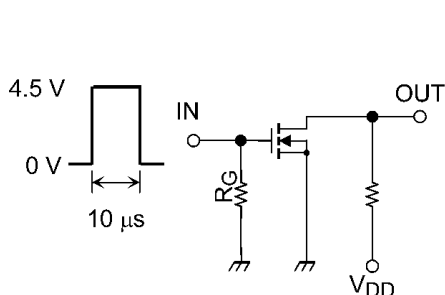
Fig. 5.3.1 Test Circuit of Switching Time
