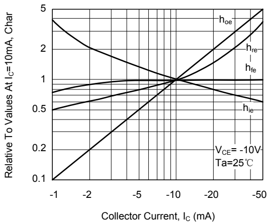
Common Emitter Characteristics
