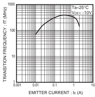
Fig.7 Transition Frequency
