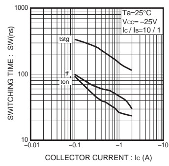
Fig.9 Switching Time
