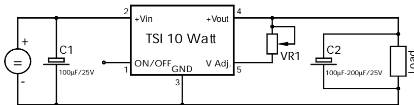
Output Voltage Adjustment Connection
