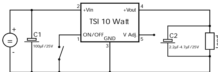
Remote ON/OFF Connection
