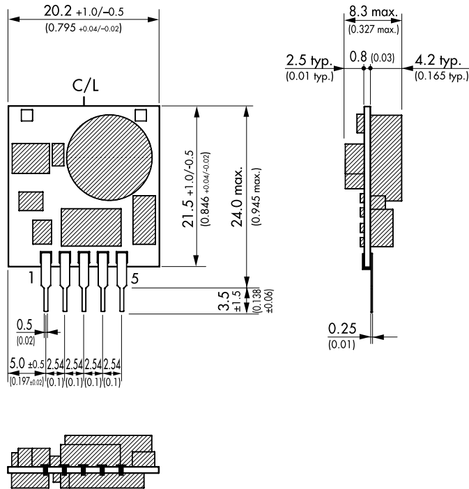
SIP package
