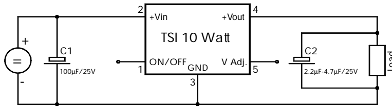
Normal Connection (Standard)
