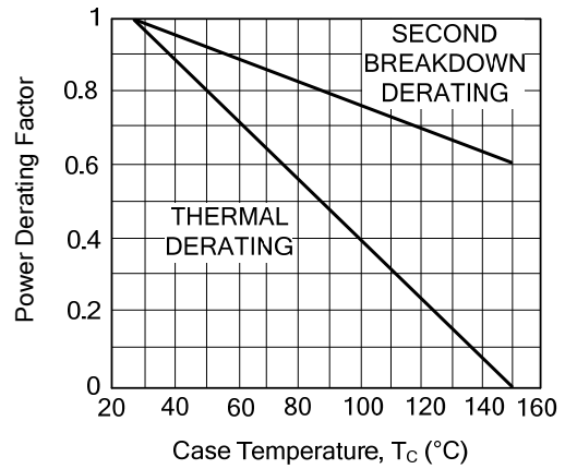
Fig. 9 Forward Bias Power Derating
