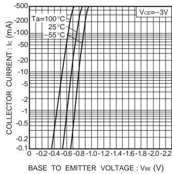
Fig.1 Grounded emitter propagation
