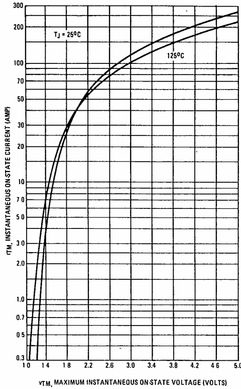
FIGURE 5 – MAXIMUM ON-STATE CHARACTERISTICS
