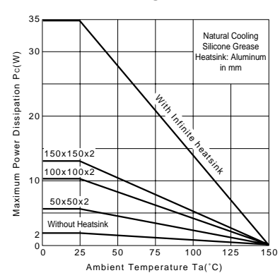
P_C-T_a Derating
