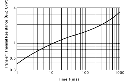
\theta_{j-a}-t Characteristics
