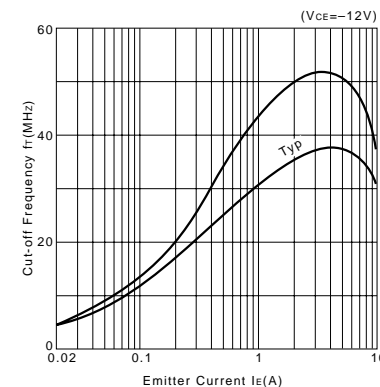
f r -I E Characteristics (Typical)
