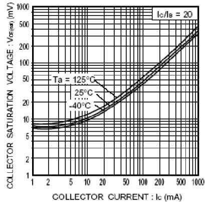
Fig.3 Collector-emitter saturation voltage vs. collector current ( I )
