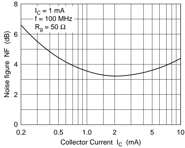
Noise Figure vs. Collector Current
