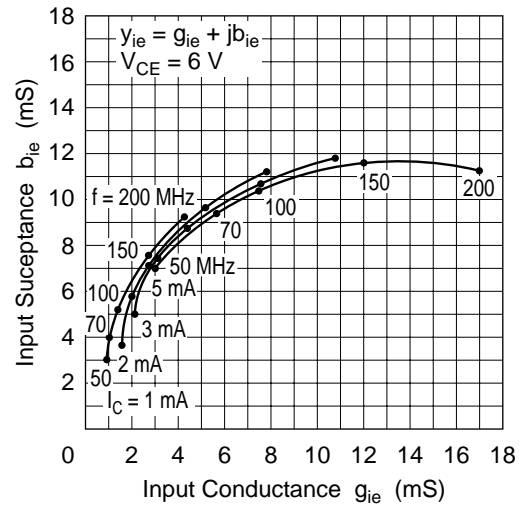
Input Admittance Characteristics
