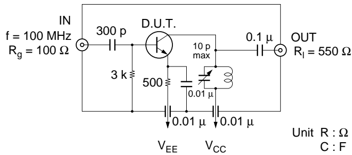
100 MHz Power Gain Test Circuit
