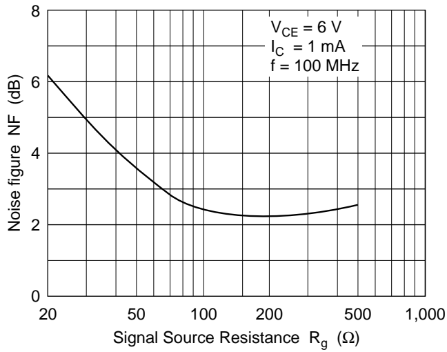
Noise Figure vs. Signal Source Resistance
