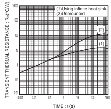
Fig.9 Transient thermal resistance
