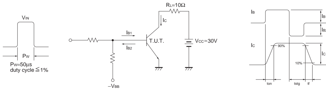
Fig.10 Switching characteristic circuit
