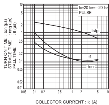
Fig.7 Switching characteristics
