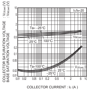
Fig.4 Collector-emitter saturation voltage Base-emitter saturation voltage—collector current
