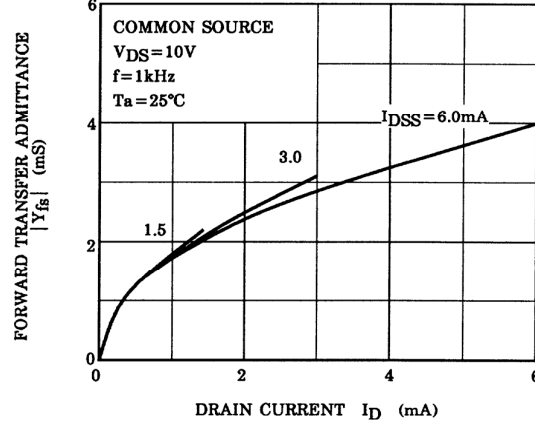
|Yfs| - ID
