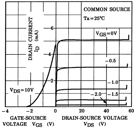
STATIC CHARACTERISTIC
