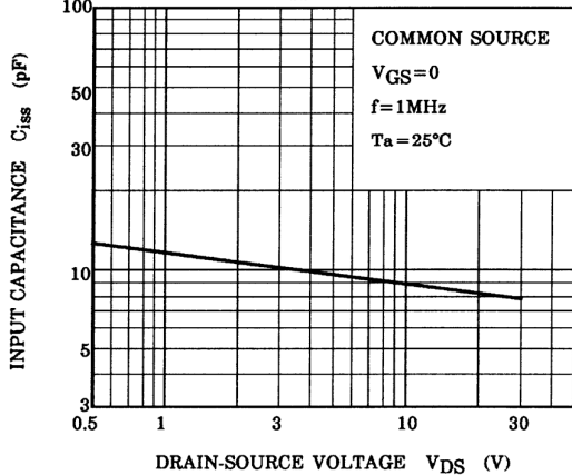
Ciss - VDS
