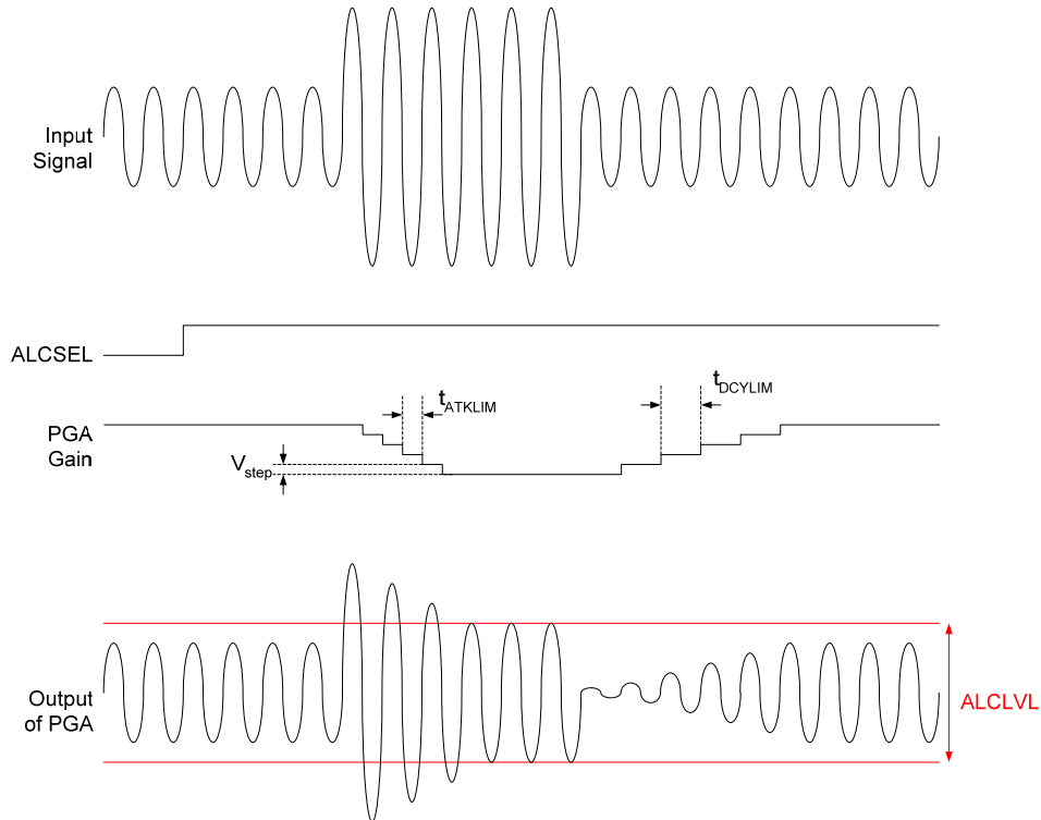
Figure 19 ALC Limiter Mode Operation
