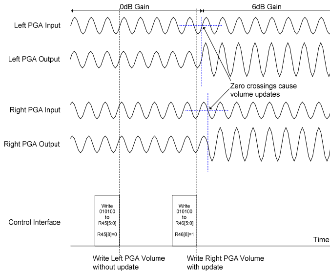
Figure 13 Volume Update Using Zero Cross Detection
