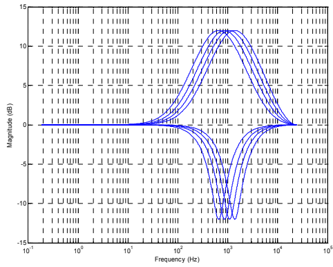
Figure 62 EQ Band 3 – Peak Filter Centre Frequencies, EQ3BW=0
