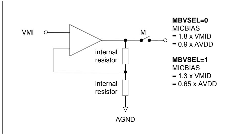
Figure 16 Microphone Bias Schematic
