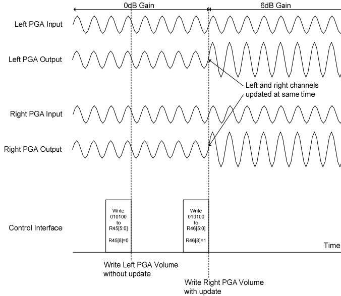
Figure 11 Simultaneous Left and Right Volume Updates
