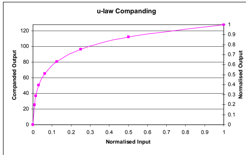
Figure 41 u-Law Comanding
