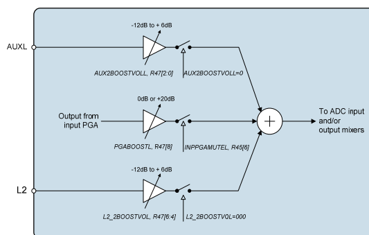
Figure 15 Input Boost Stage
