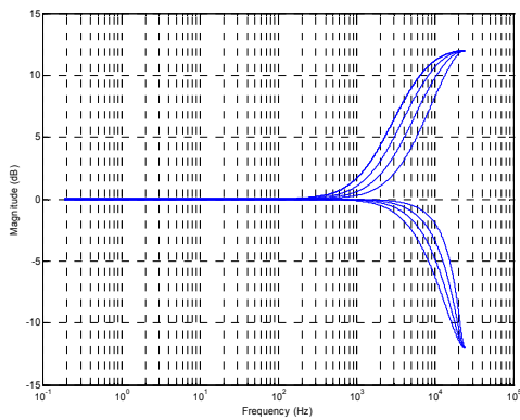
Figure 68 EQ Band 5 High Frequency Shelf Filter Cut-offs
