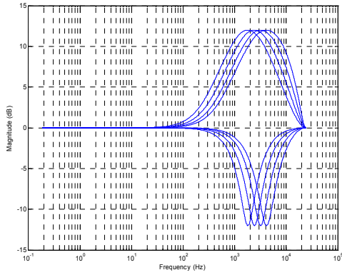
Figure 65 EQ Band 4 – Peak Filter Centre Frequencies, EQ3E
