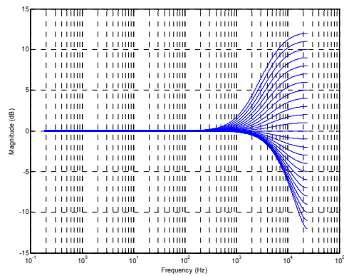
Figure 69 EQ Band 5 Gains for Lowest Cut-off Frequency
