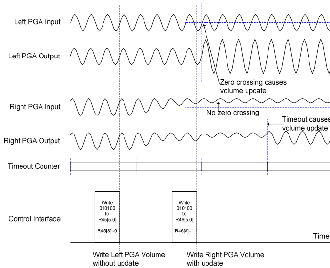
Figure 14 Volume Update after Timeout
