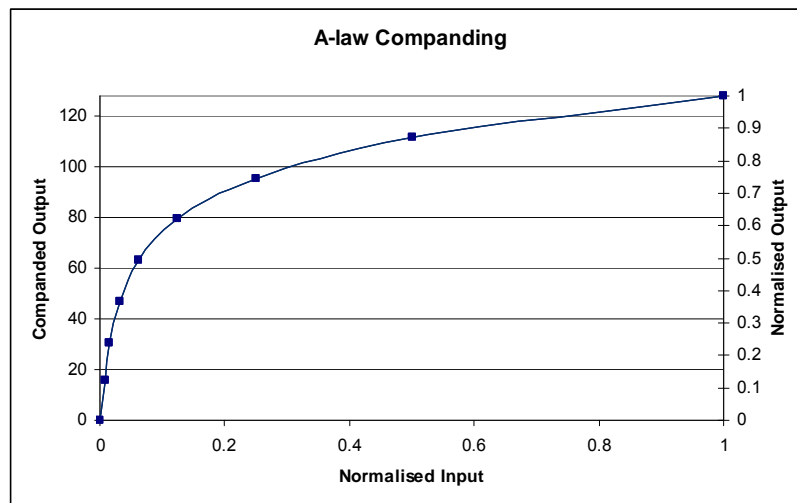
Figure 42 A-Law Comanding
