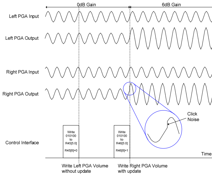
Figure 12 Click Noise During Volume Update
