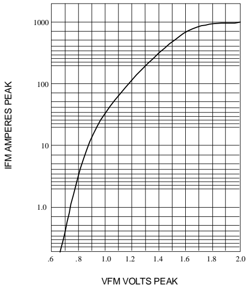
Fig. 1-TYPICAL INSTANTANEOUS FORWARD CHARACTERISTICS AT T_J = 25\text{ }^{\circ}\text{C}
