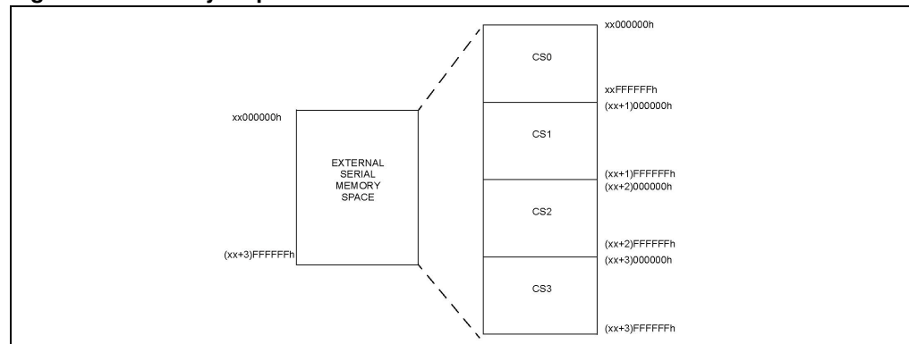
Figure 13. Memory map
