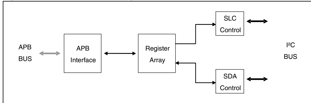
Figure 15. I 2 C Controller block diagram
