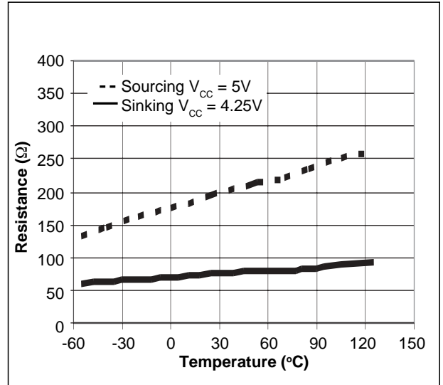
Figure 8. RESET Output Resistance vs. Temperature
