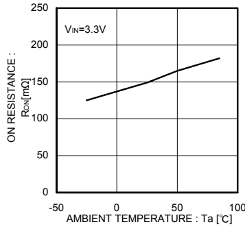
Fig.11 ON resistance
