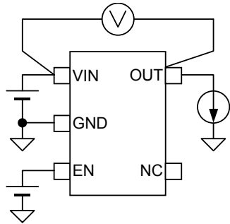
ON resistance
