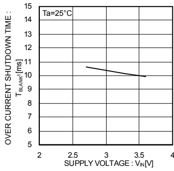
Fig.16 Over current shutdown time
