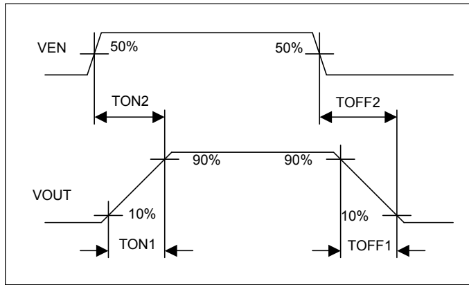
Fig.2 Switch Turn on / off time
