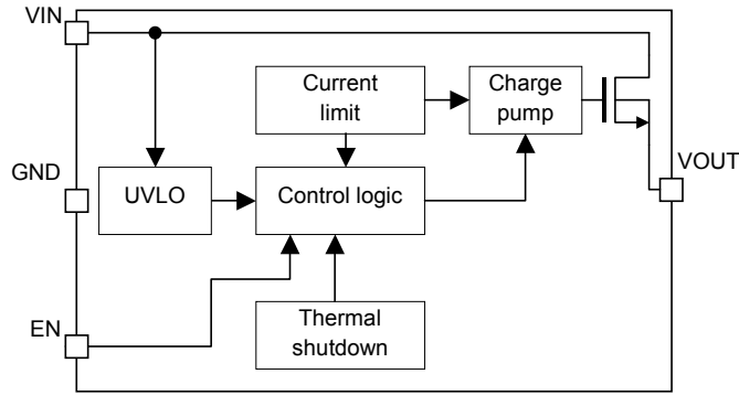
Fig.38 Block diagram
