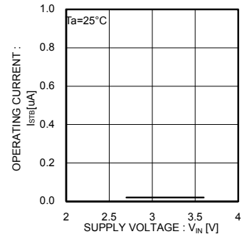
Fig.6 Operating current EN Disable
