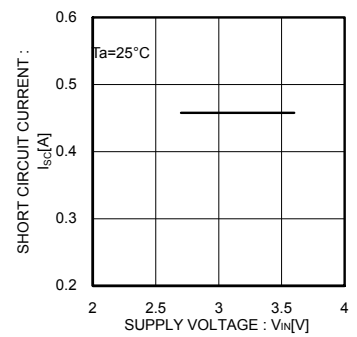
Fig.12 Short circuit output current (BD2202G)
