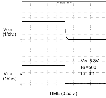
Fig.29 Output turn off response
