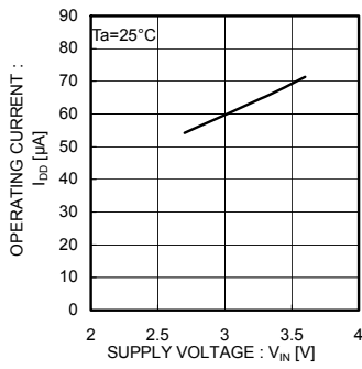
Fig.4 Operating current EN Enable
