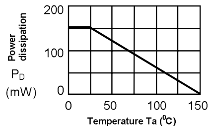
Figure 10 Power dissipation of an SOT-23-5 Package (Free-Air)
