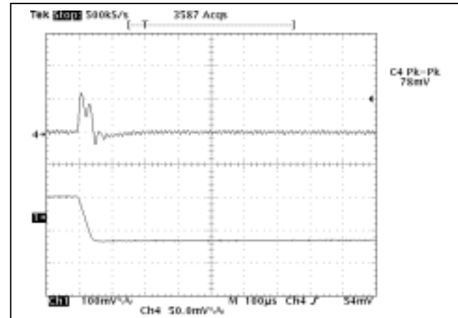
Figure 17. 3.3V Transient Response 50% to 75% step at V_{IN} = 48Vdc , T_A = 25^\circ C , di/dt = 0.1A/\mu s , C_O = 0 .
