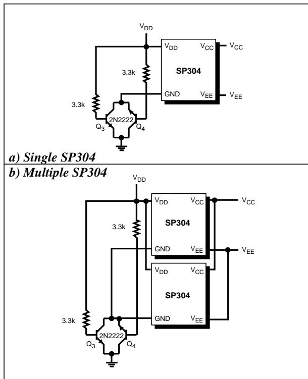
Figure 1. Isolating the SP304 from Ground.
