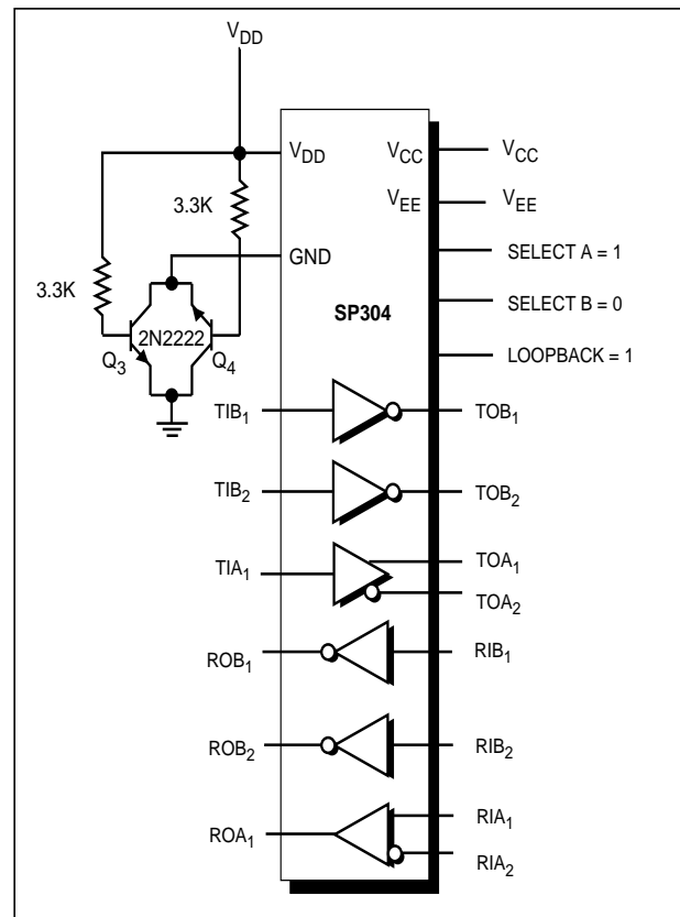
Figure 2. Typical Circuit
