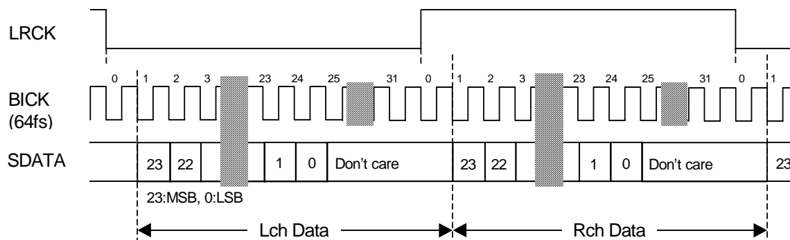
Figure 4. Mode 3 Timing
