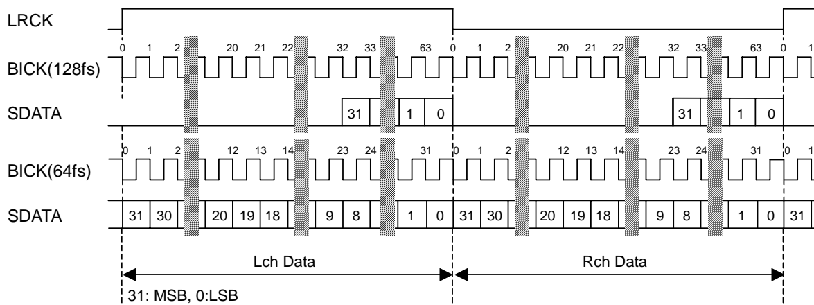
Figure 5. Mode 5 Timing
