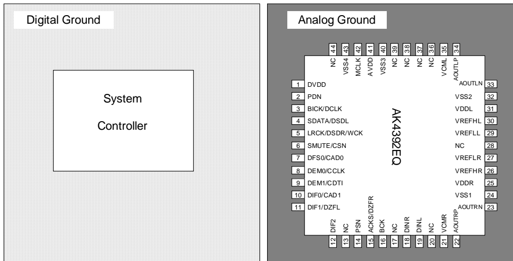
Figure 18. Ground Layout
