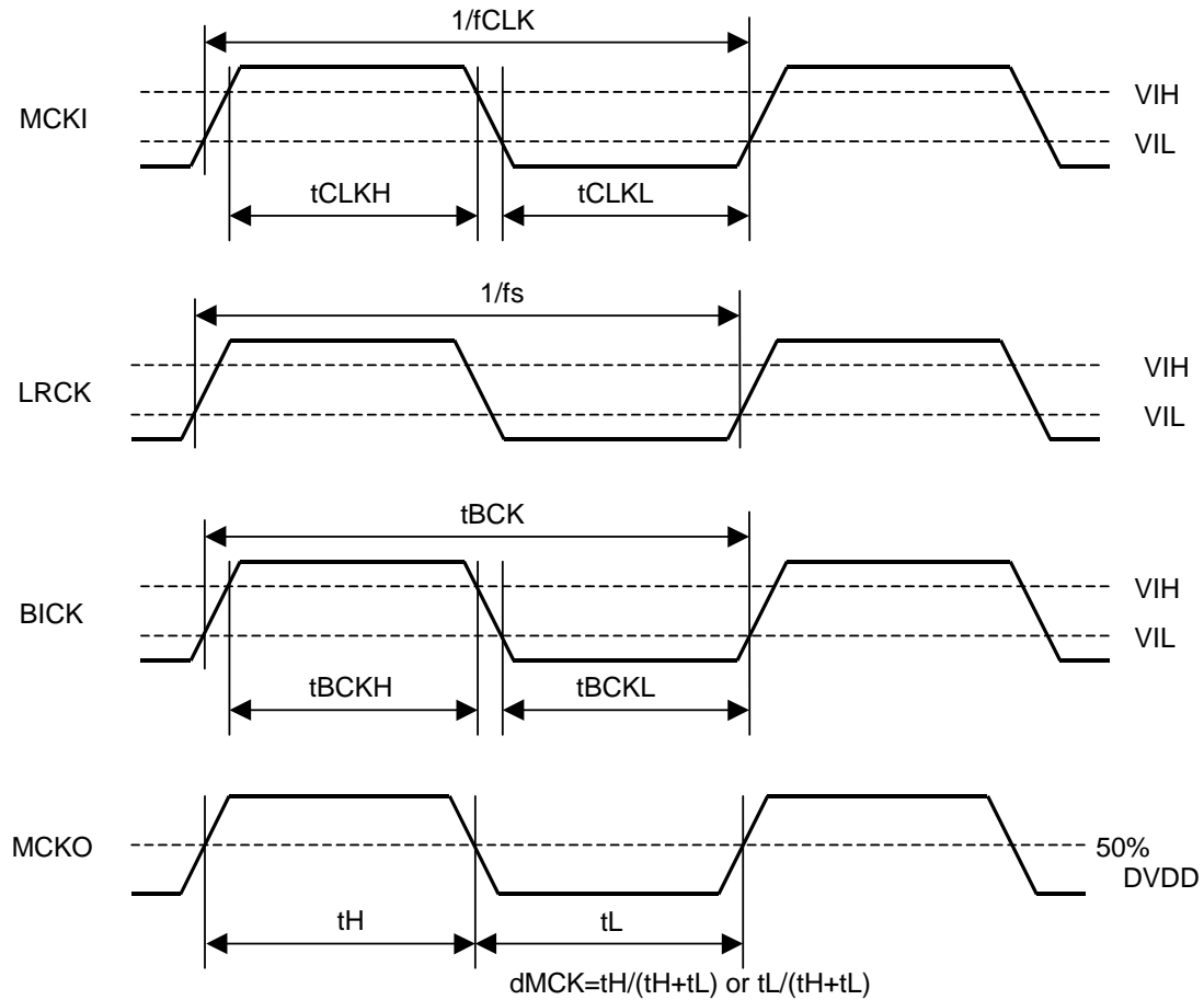
Figure 4. Clock Timing
