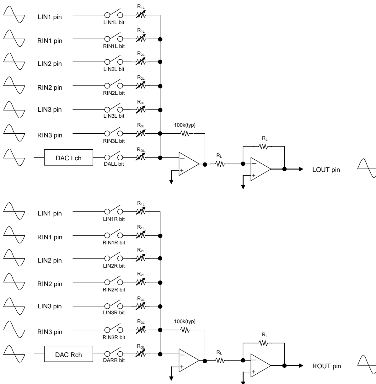
Figure 26. Summation circuit for stereo line output
