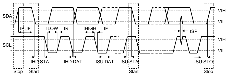
Figure 9. I²C Bus Mode Timing
