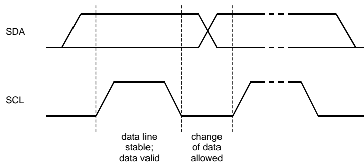
Figure 22. Bit transfer on the I 2 C-bus
