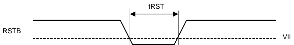
Reset Timing
