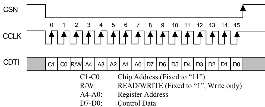
Figure 15. Control I/F Timing
