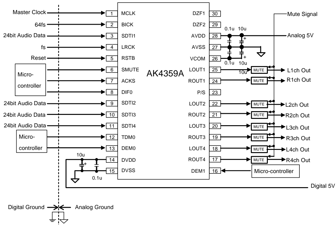
Figure 23. Typical Connection Diagram (Parallel Control Mode)
