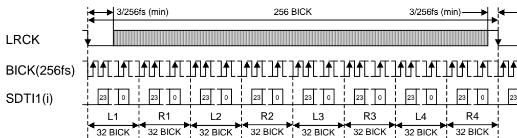
Figure 6. Mode 6 Timing
