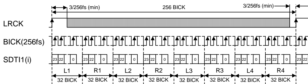
Figure 5. Mode 5 Timing
