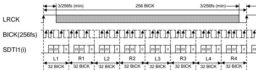
Figure 7. Mode 7 Timing
