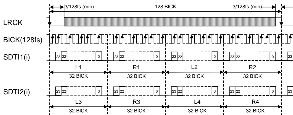
Figure 9. Mode 9 Timing
