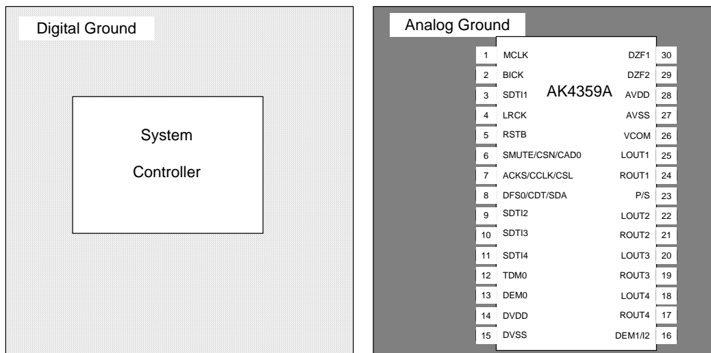
Figure 25. Ground Layout
