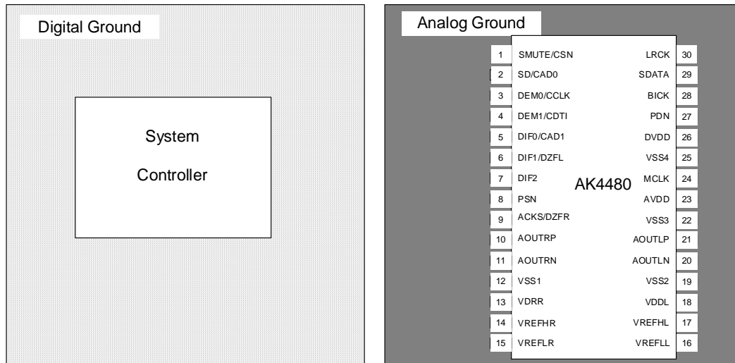
Figure 18. Ground Layout
