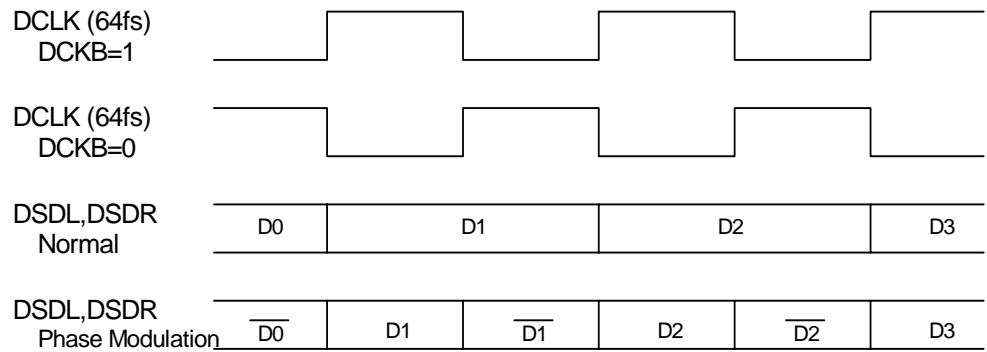
Figure 8. DSD Mode Timing
