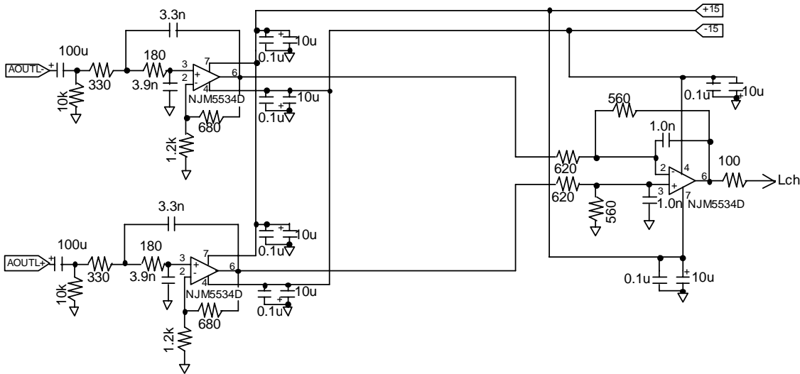
Figure 20. External LPF Circuit Example 2 for PCM
