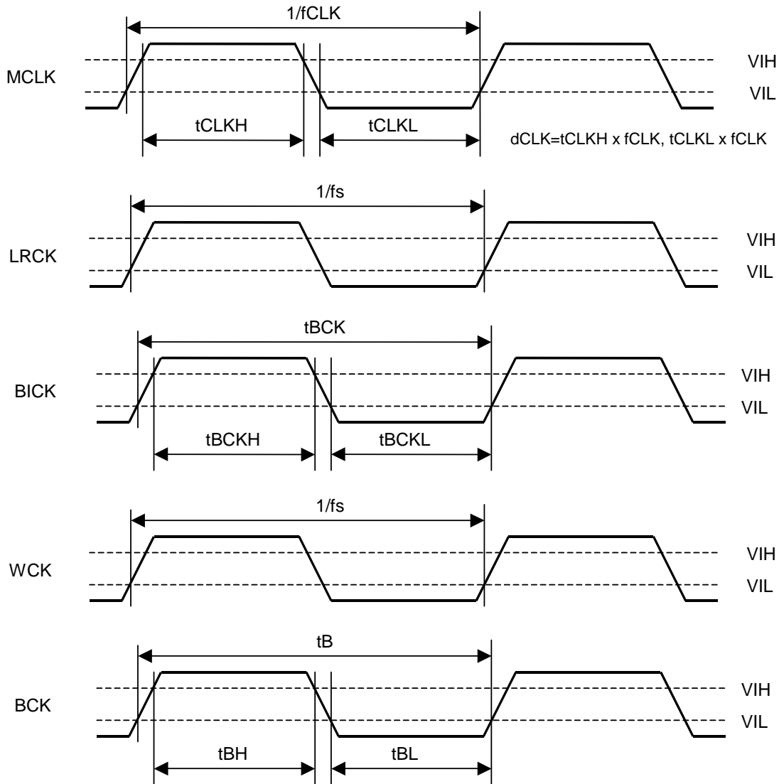
Clock Timing
