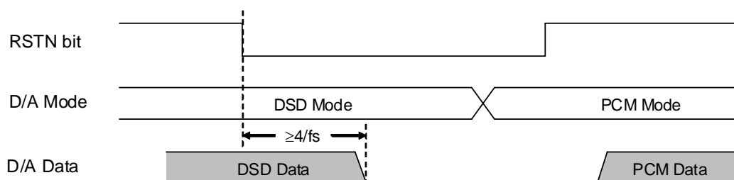
Figure 11. D/A Mode Switching Timing (DSD to PCM)
