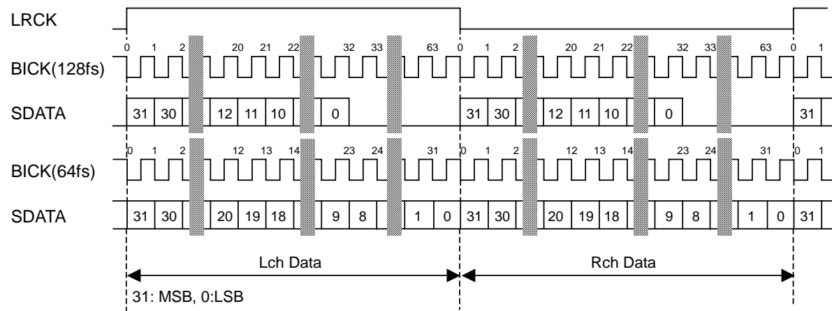
Figure 6. Mode 6 Timing
