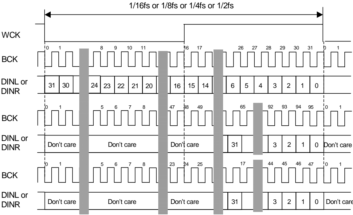
Figure 9. EX DF I/F Mode Timing
