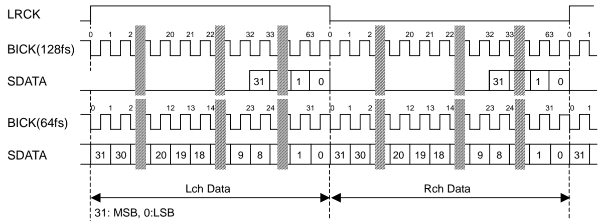
Figure 5. Mode 5 Timing
