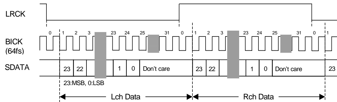
Figure 4. Mode 3 Timing
