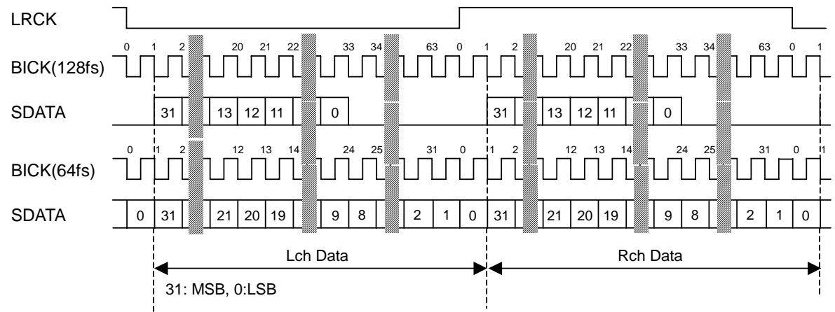
Figure 7. Mode 7 Timing
