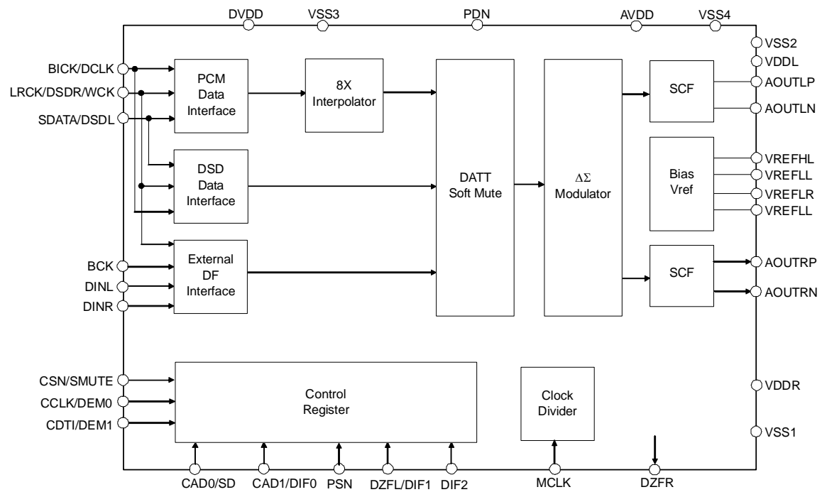
Block Diagram
