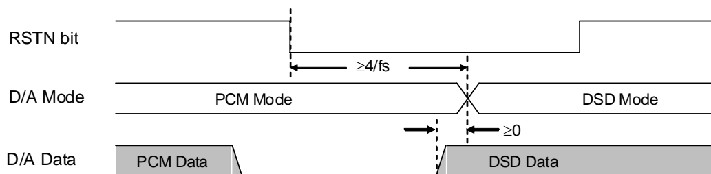
Figure 10. D/A Mode Switching Timing (PCM to DSD)
