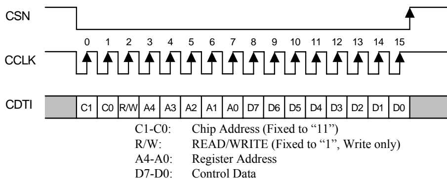
Figure 21. Control I/F Timing
