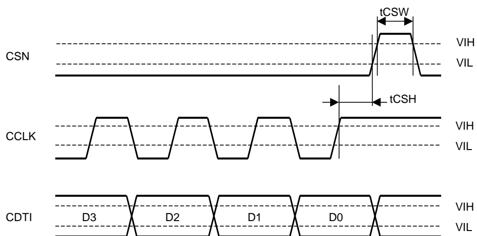
Figure 4. WRITE Data Input Timing
