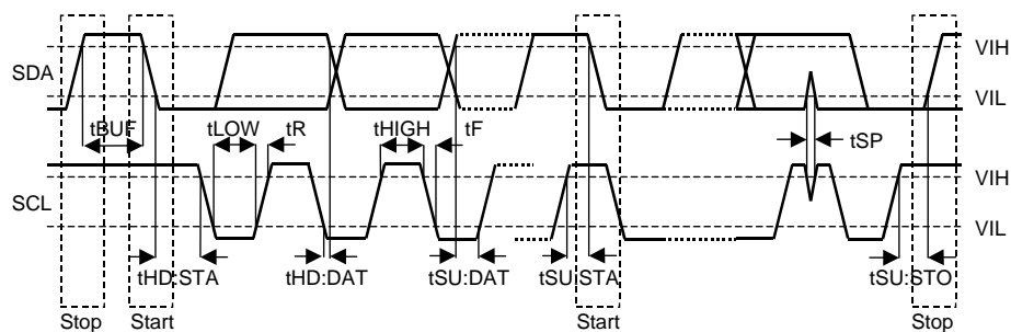
Figure 5. I 2 C Bus mode Timing
