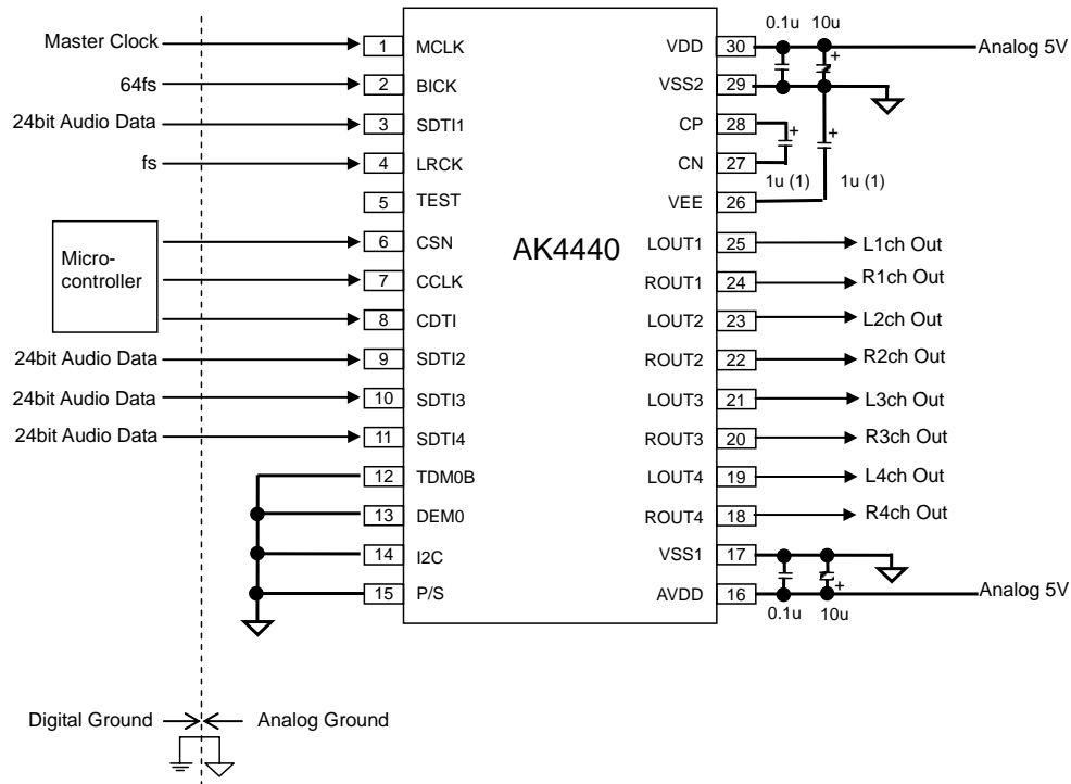
Figure 30. Typical Connection Diagram (3-wire Serial Control Mode)
