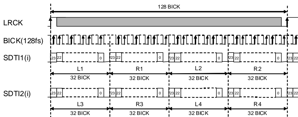
Figure 13. Mode 8 Timing
