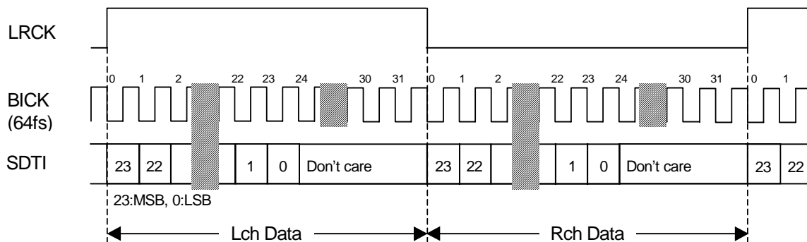
Figure 8. Mode 2 Timing
