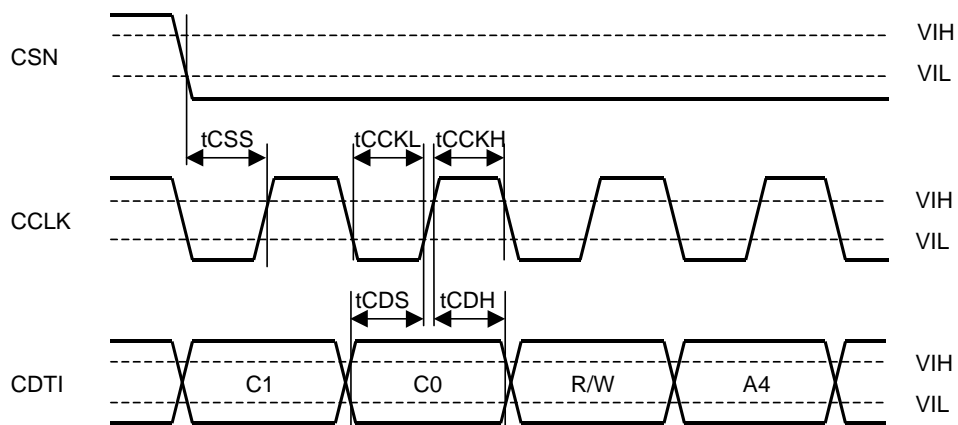
Figure 3. WRITE Command Input Timing
