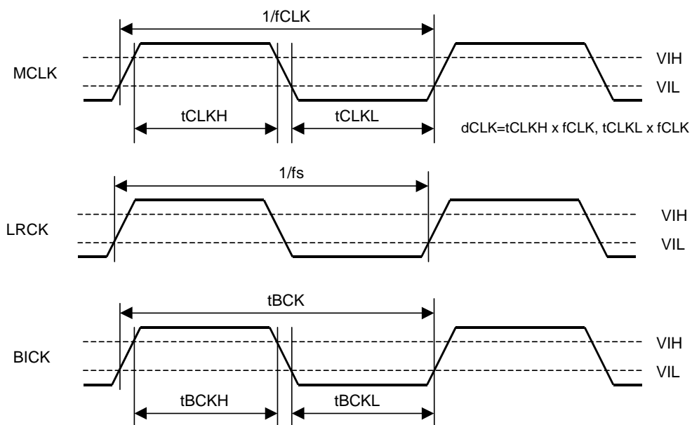
Figure 1. Clock Timing
