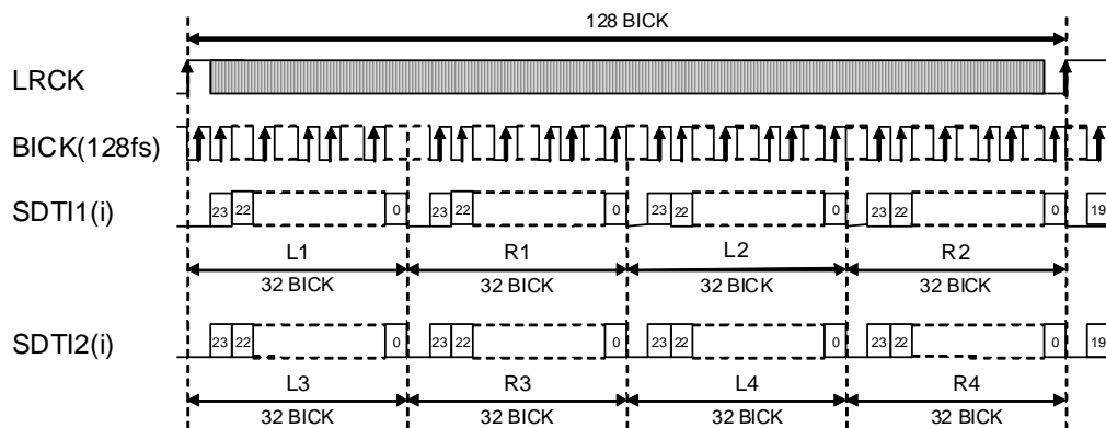
Figure 15. Mode 10 Timing
