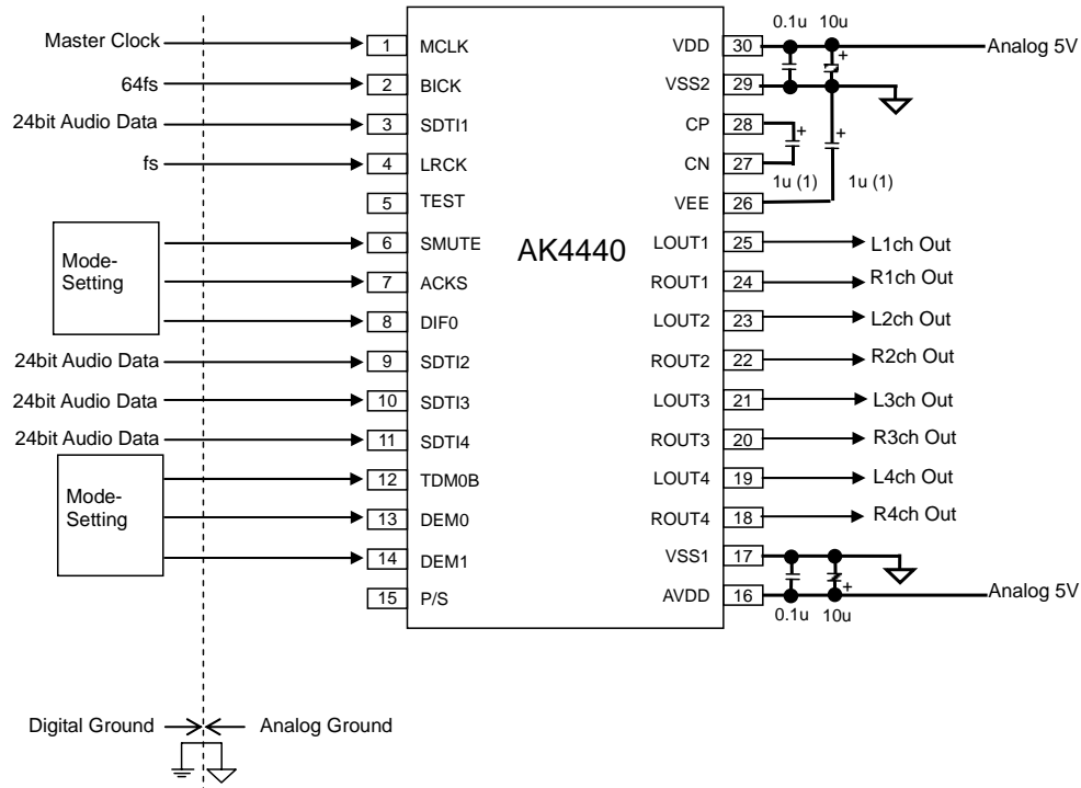
Figure 29. Typical Connection Diagram (Parallel Control Mode)
