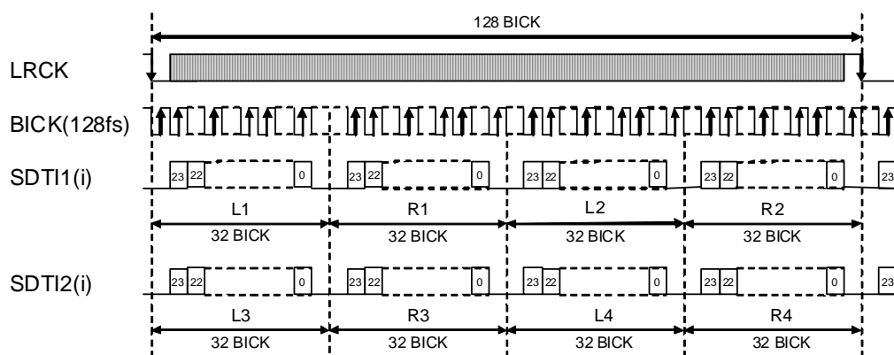
Figure 14. Mode 9 Timing
