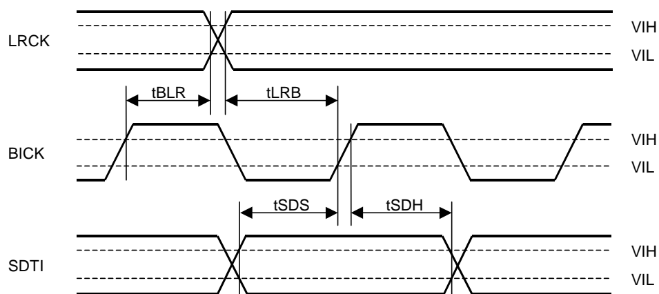
Figure 2. Audio Serial Interface Timing
