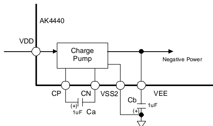
Figure 16. Negative Power Generation Circuit
