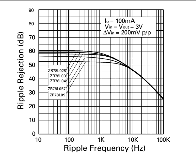
Ripple Rejection vs. Ripple Frequency
