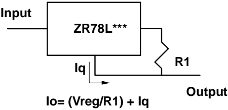
Current Regulator
