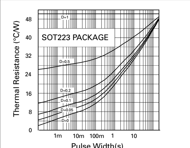
Thermal Resistance v Pulse Width
