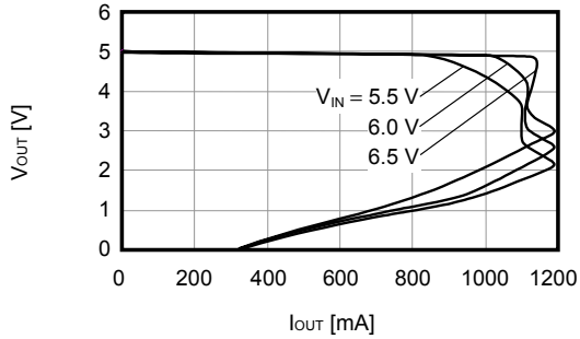
S-1170B50 (Ta = 25°C)
