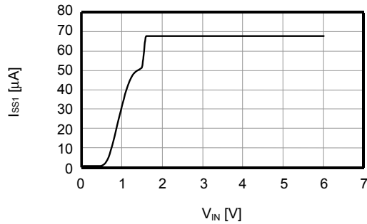
S-1170B50 ( T_a = 25^\circ\text{C} )
