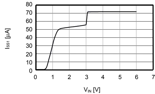
S-1170B30 ( T_a = 25^\circ\text{C} )
