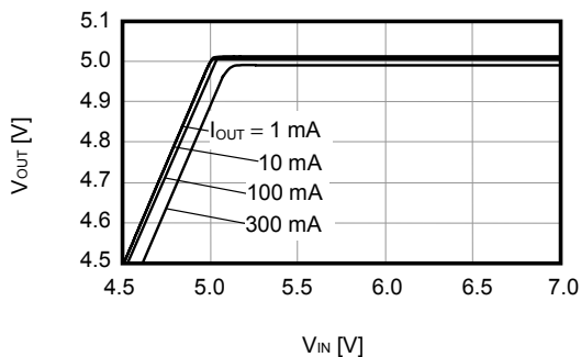
S-1170B50 (Ta = 25°C)
