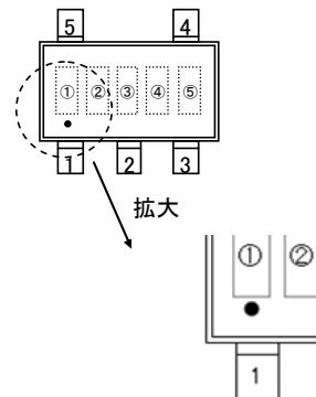
SOT-25(Under dot 仕様)
