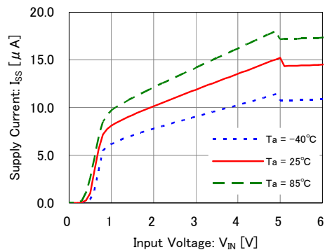
XC6501x501
