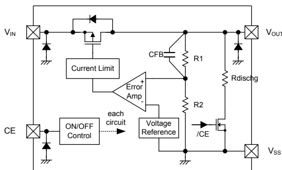
XC6501B Series
