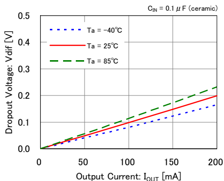
XC6501x501
