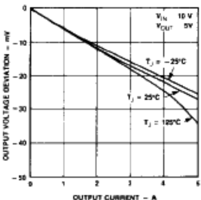
Load Regulation
