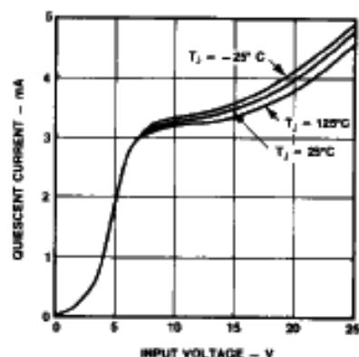
Quiescent Current
