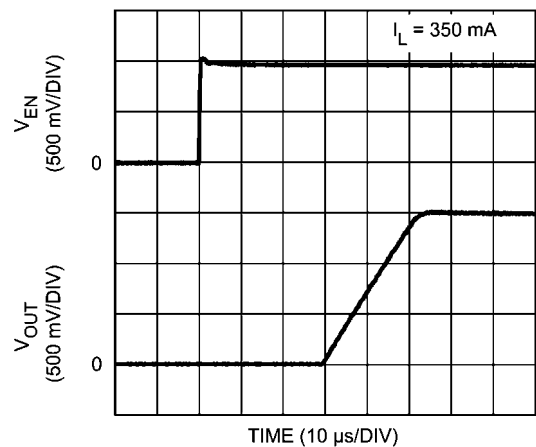
Enable Start-up Time, 1.5V Option
