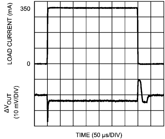
Load Transient Response, 1.5V Option
