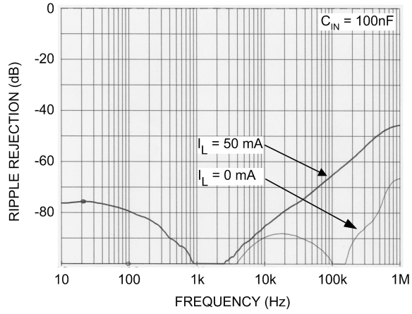
Power Supply Rejection Ratio V_{IN} , 1.5V Option
