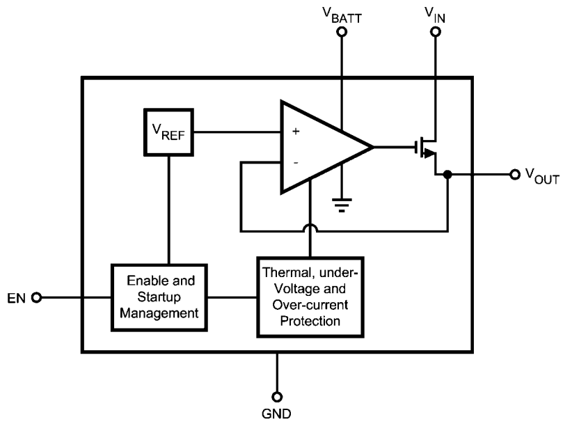
FIGURE 5: Block Diagram
