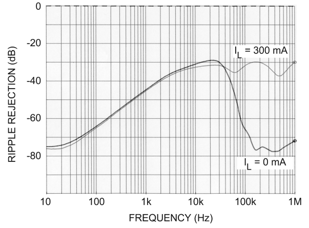
Power Supply Rejection Ratio V_{BATT} , 1.5V Option
