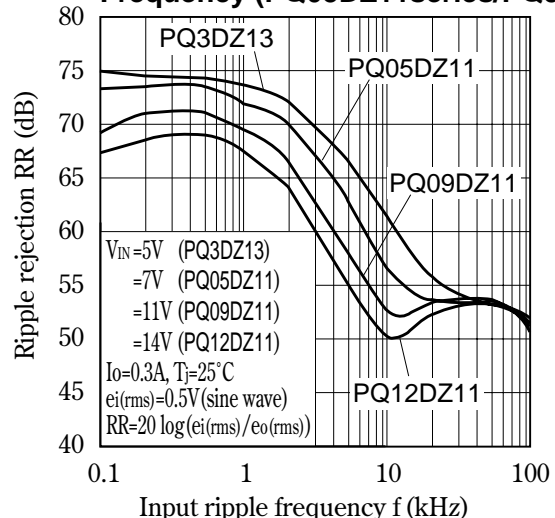
Fig.38 Ripple Rejection vs. Input Ripple Frequency (PQ05DZ11series/PQ3DZ13)
