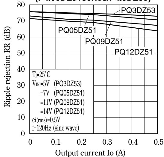
Fig.39 Ripple Rejection vs. Output Current (PQ05DZ51series/PQ3DZ53)
