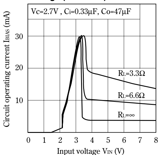
Fig.31 Circuit Operating Current vs. Input Voltage (PQ09DZ11)
