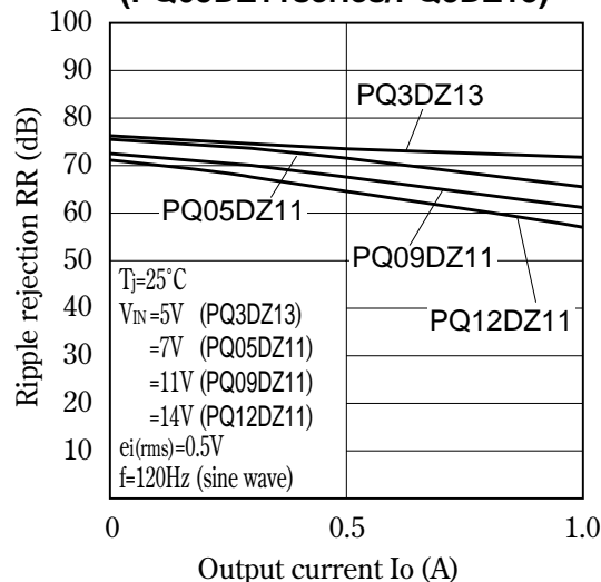
Fig.40 Ripple Rejection vs. Output Current (PQ05DZ11series/PQ3DZ13)
