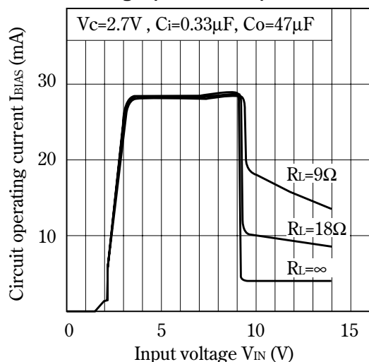
Fig.31 Circuit Operating Current vs. Input Voltage (PQ09DZ11)
