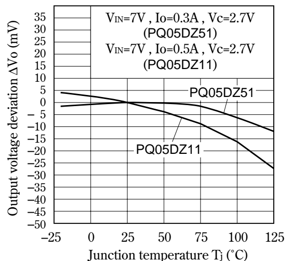
Fig.14 Output Voltage Deviation vs. Junction Temperature (PQ05DZ51/11)
