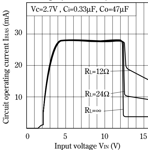
Fig.32 Circuit Operating Current vs. Input Voltage (PQ12DZ11)
