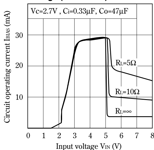
Fig.32 Circuit Operating Current vs. Input Voltage (PQ12DZ11)
