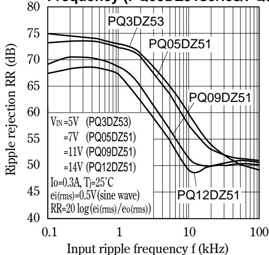
Fig.37 Ripple Rejection vs. Input Ripple Frequency (PQ05DZ51series/PQ3DZ53)
