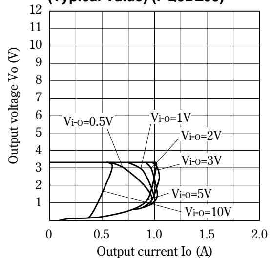
Fig. 4 Overcurrent Protection Characteristics (Typical Value) (PQ3DZ53)
