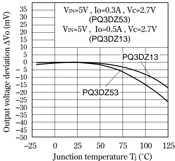
Fig.13 Output Voltage Deviation vs. Junction Temperature (PQ3DZ53/13)
