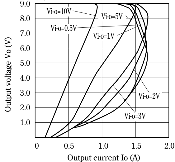
Fig.10 Overcurrent Protection Characteristics (Typical Value)(PQ09DZ11)
