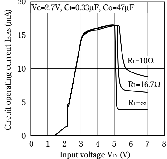
Fig.26 Circuit Operating Current vs. Input Voltage (PQ05DZ51)
