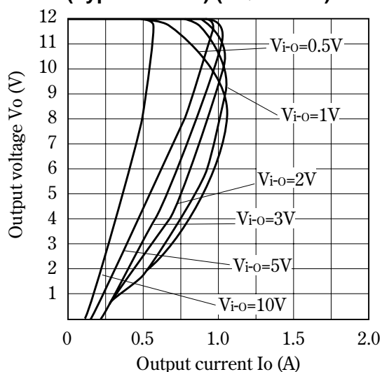
Fig.10 Overcurrent Protection Characteristics (Typical Value)(PQ09DZ11)
