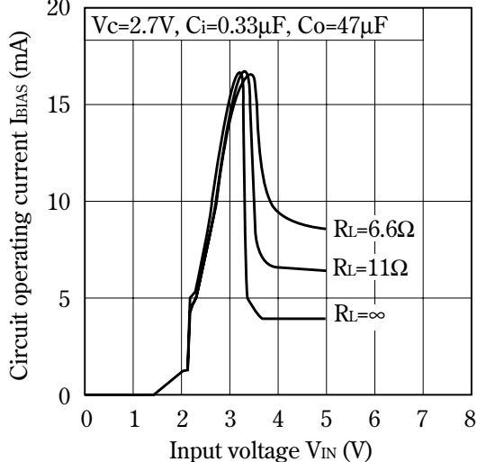
Fig.25 Circuit Operating Current vs. Input Voltage (PQ3DZ53)
